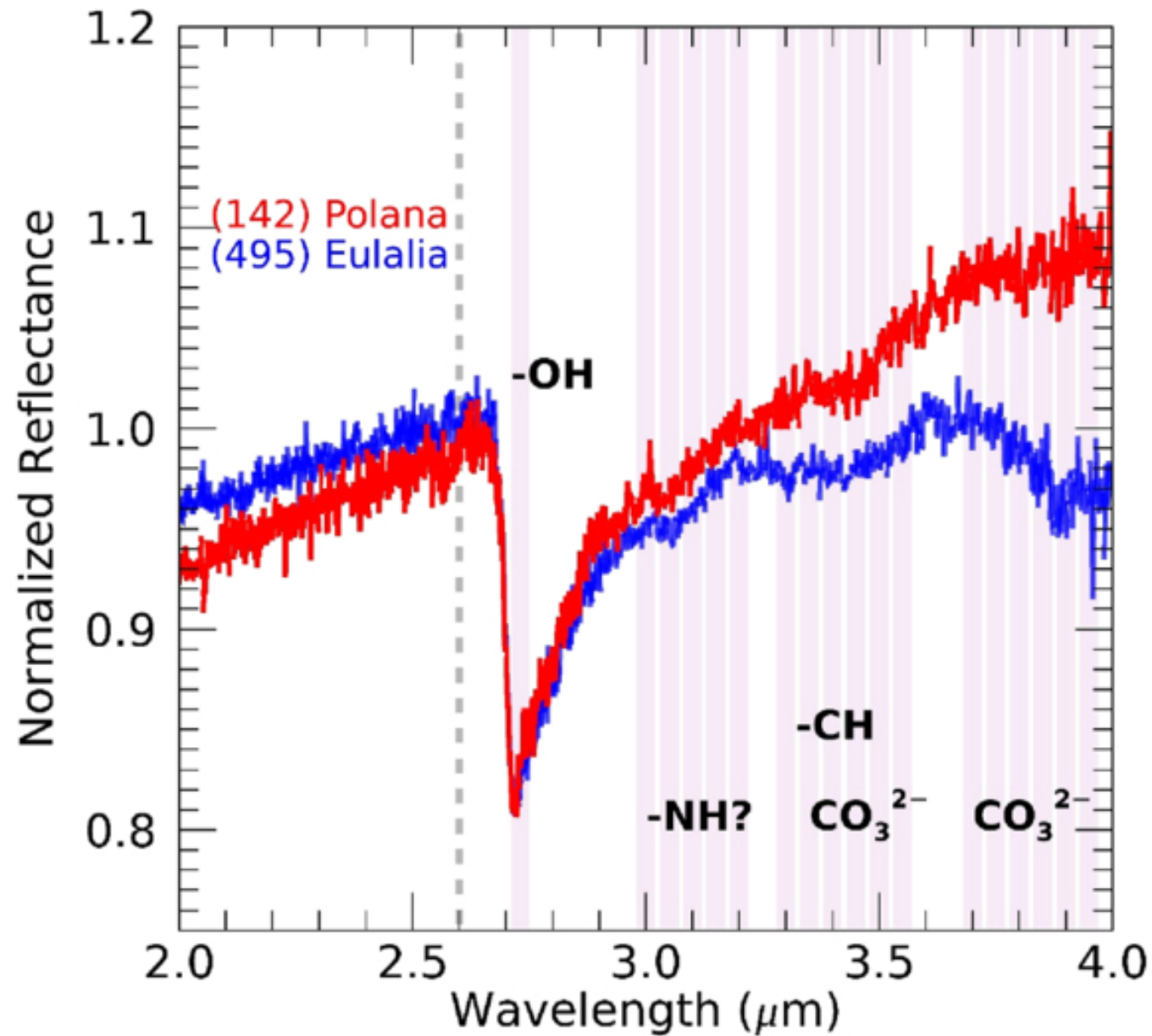
Figure 8. from Lucas T. McClure et al 2026 Planet. Sci. J. 7 doi:10.3847/PSJ/ae8e7a https://dx.doi.org/10.3847/PSJ/ae8e7a © 2026. The Author(s). Published by the American Astronomical Society.
