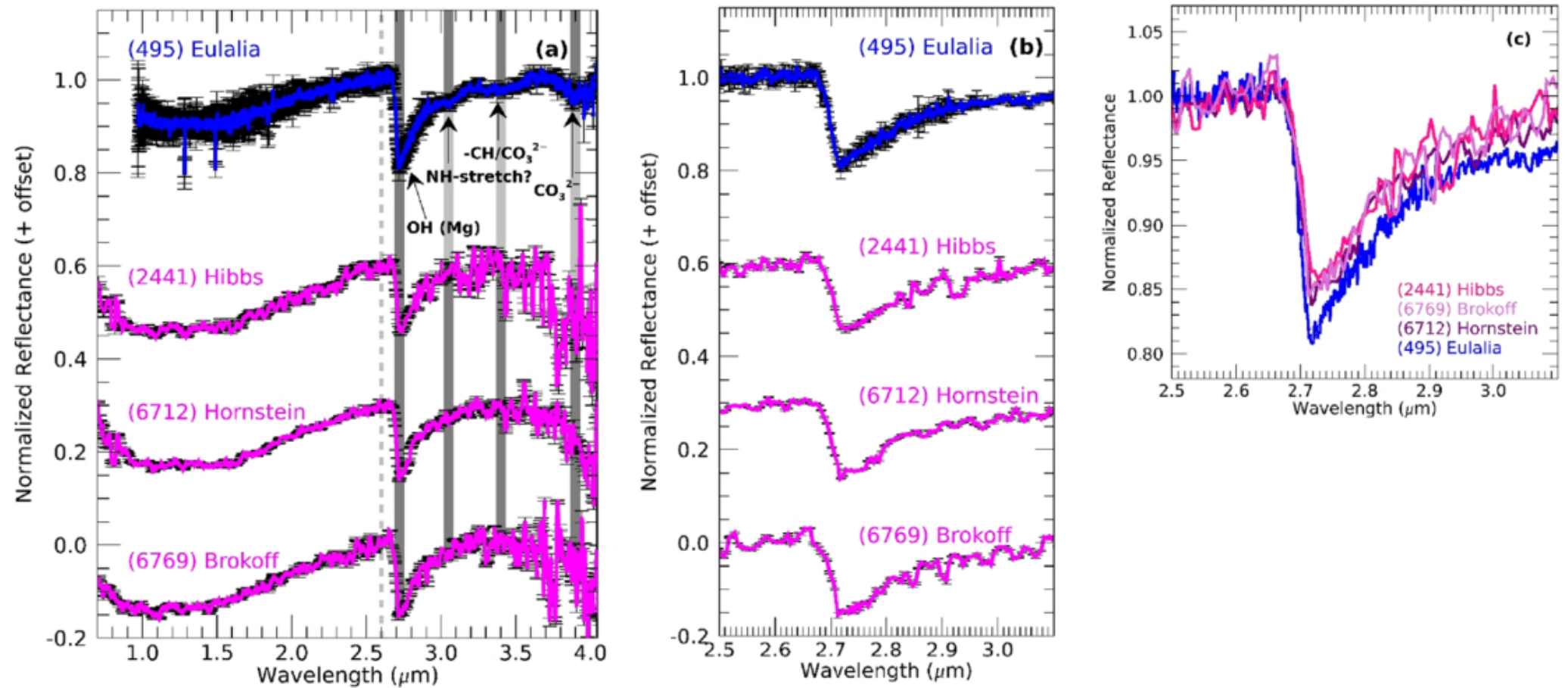
Figure 3. from Lucas T. McClure et al 2026 Planet. Sci. J. 7 doi:10.3847/PSJ/ae8e7a https://dx.doi.org/10.3847/PSJ/ae8e7a © 2026. The Author(s). Published by the American Astronomical Society.
