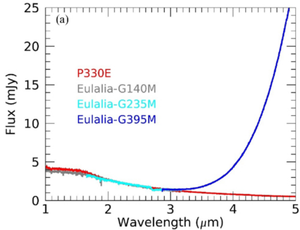
Figure 2. from Lucas T. McClure et al 2026 Planet. Sci. J. 7 doi:10.3847/PSJ/ae8e7a https://dx.doi.org/10.3847/PSJ/ae8e7a © 2026. The Author(s). Published by the American Astronomical Society.
