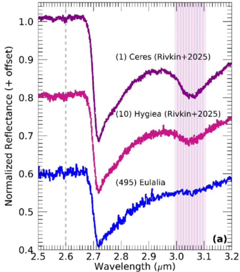
Figure 10. from Lucas T. McClure et al 2026 Planet. Sci. J. 7 doi:10.3847/PSJ/ae8e7a https://dx.doi.org/10.3847/PSJ/ae8e7a © 2026. The Author(s). Published by the American Astronomical Society.
