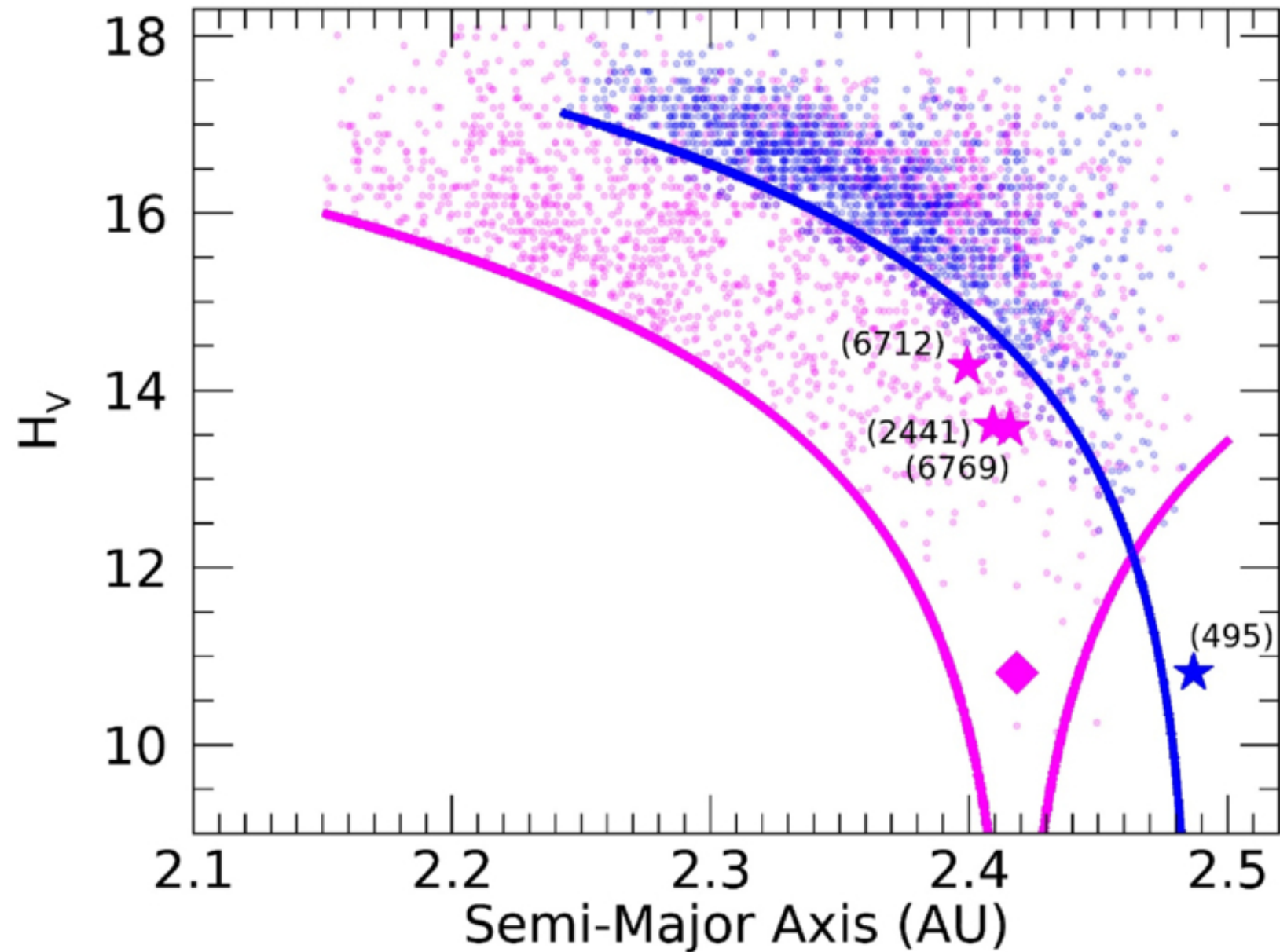
Figure 1. from Lucas T. McClure et al 2026 Planet. Sci. J. 7 doi:10.3847/PSJ/ae8e7a https://dx.doi.org/10.3847/PSJ/ae8e7a © 2026. The Author(s). Published by the American Astronomical Society.
