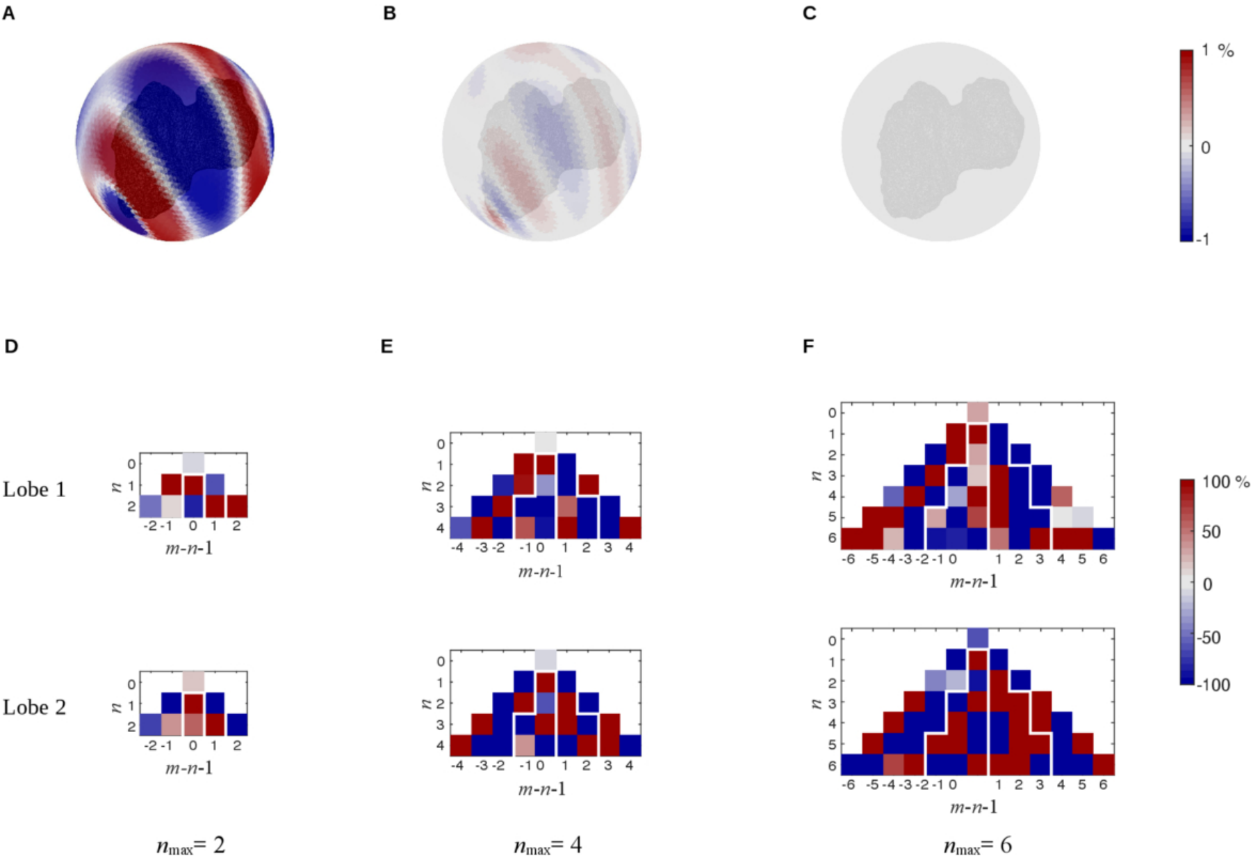
Figure 5. from Xuanyu Hu 2026 Planet. Sci. J. 7 doi:10.3847/PSJ/ae8d2b https://dx.doi.org/10.3847/PSJ/ae8d2b © 2026. The Author(s). Published by the American Astronomical Society.
