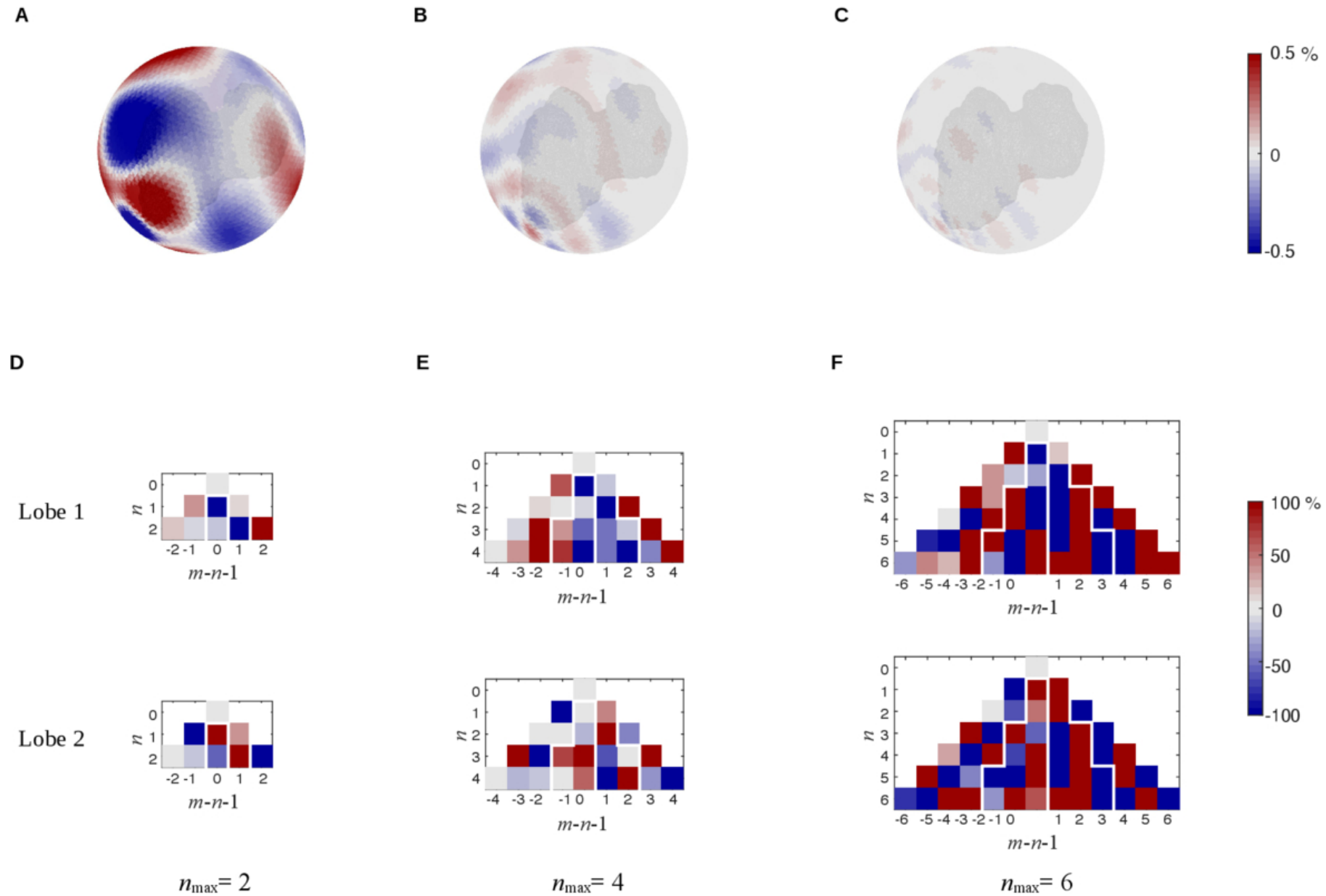
Figure 4. from Xuanyu Hu 2026 Planet. Sci. J. 7 doi:10.3847/PSJ/ae8d2b https://dx.doi.org/10.3847/PSJ/ae8d2b © 2026. The Author(s). Published by the American Astronomical Society.
