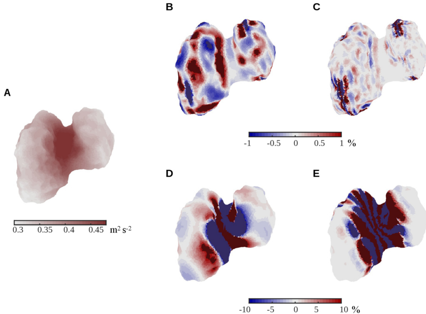
Figure 3. from Xuanyu Hu 2026 Planet. Sci. J. 7 doi:10.3847/PSJ/ae8d2b https://dx.doi.org/10.3847/PSJ/ae8d2b © 2026. The Author(s). Published by the American Astronomical Society.
