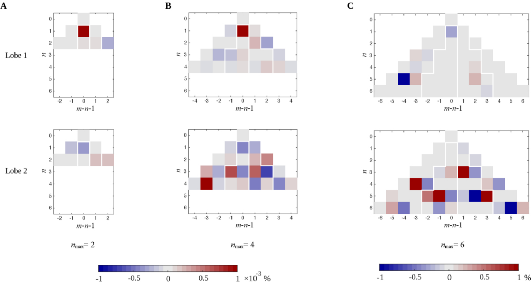
Figure 10. from Xuanyu Hu 2026 Planet. Sci. J. 7 doi:10.3847/PSJ/ae8d2b https://dx.doi.org/10.3847/PSJ/ae8d2b © 2026. The Author(s). Published by the American Astronomical Society.
