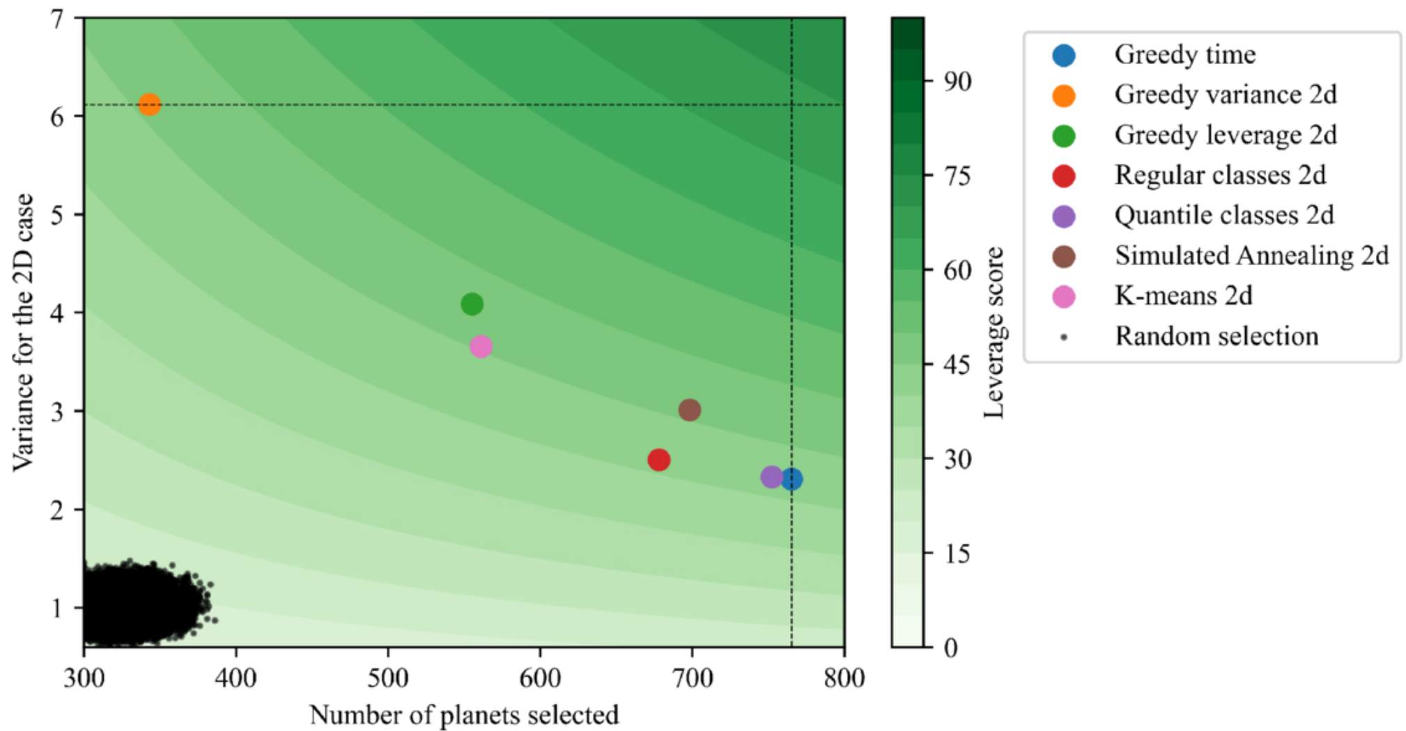
Figure 5. from Emilie Panek et al 2026 Planet. Sci. J. 7 doi:10.3847/PSJ/ae8d1a https://dx.doi.org/10.3847/PSJ/ae8d1a © 2026. The Author(s). Published by the American Astronomical Society.
