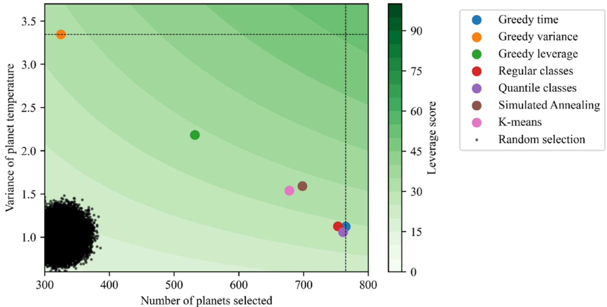
Figure 4. from Emilie Panek et al 2026 Planet. Sci. J. 7 doi:10.3847/PSJ/ae8d1a https://dx.doi.org/10.3847/PSJ/ae8d1a © 2026. The Author(s). Published by the American Astronomical Society.
