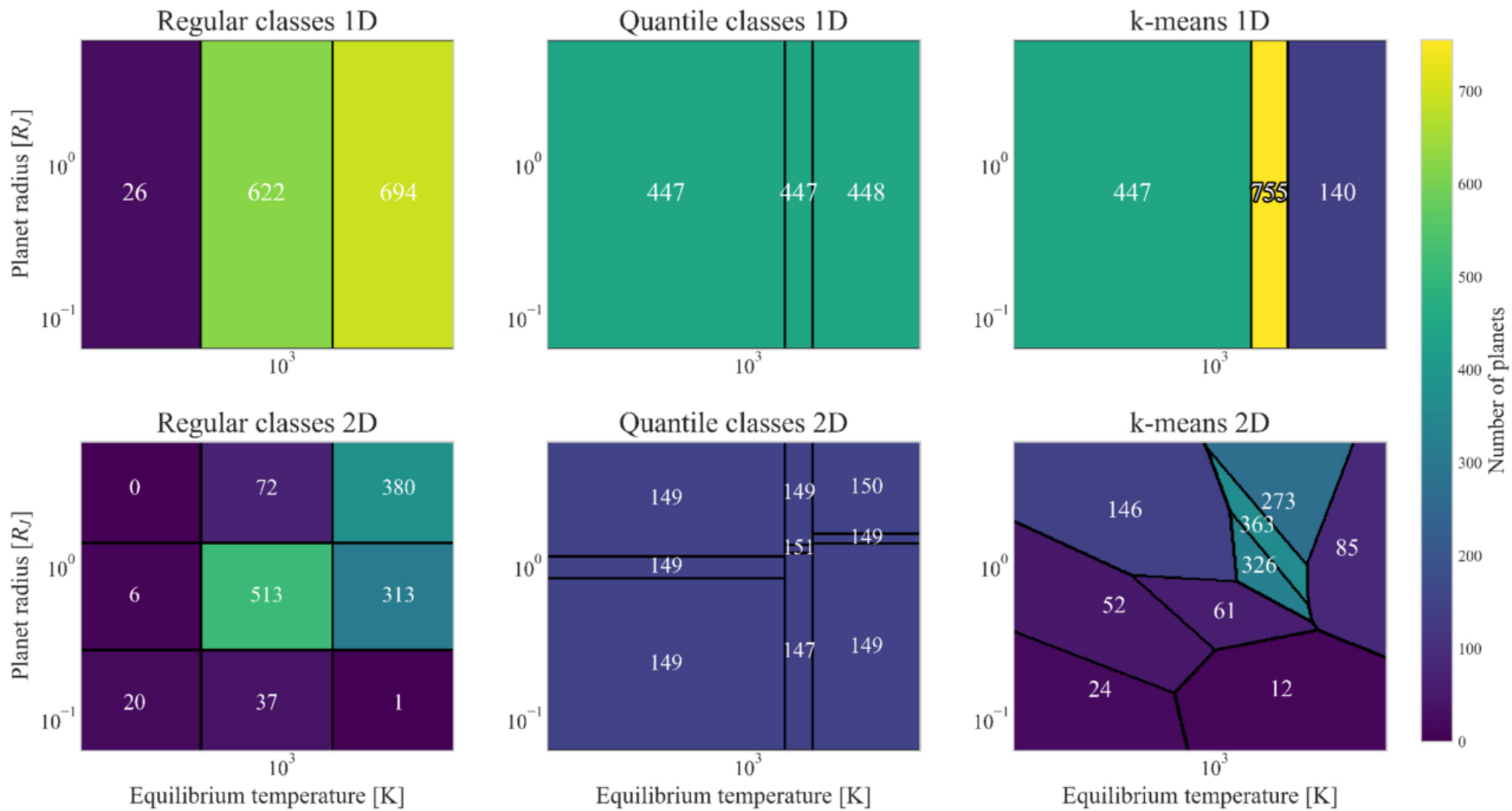
Figure 3. from Emilie Panek et al 2026 Planet. Sci. J. 7 doi:10.3847/PSJ/ae8d1a https://dx.doi.org/10.3847/PSJ/ae8d1a © 2026. The Author(s). Published by the American Astronomical Society.
