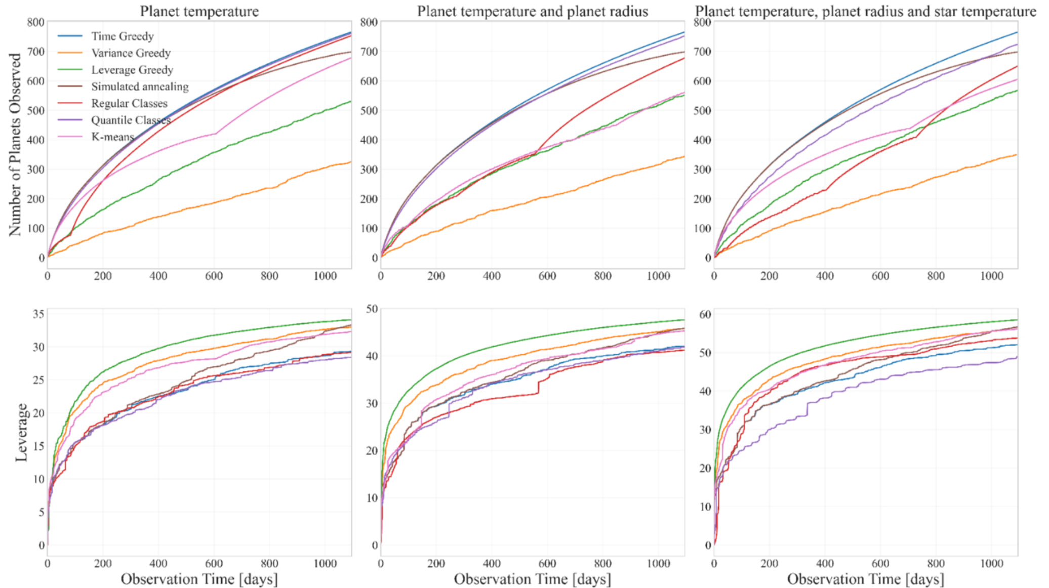
Figure 11. from Emilie Panek et al 2026 Planet. Sci. J. 7 doi:10.3847/PSJ/ae8d1a https://dx.doi.org/10.3847/PSJ/ae8d1a © 2026. The Author(s). Published by the American Astronomical Society.
