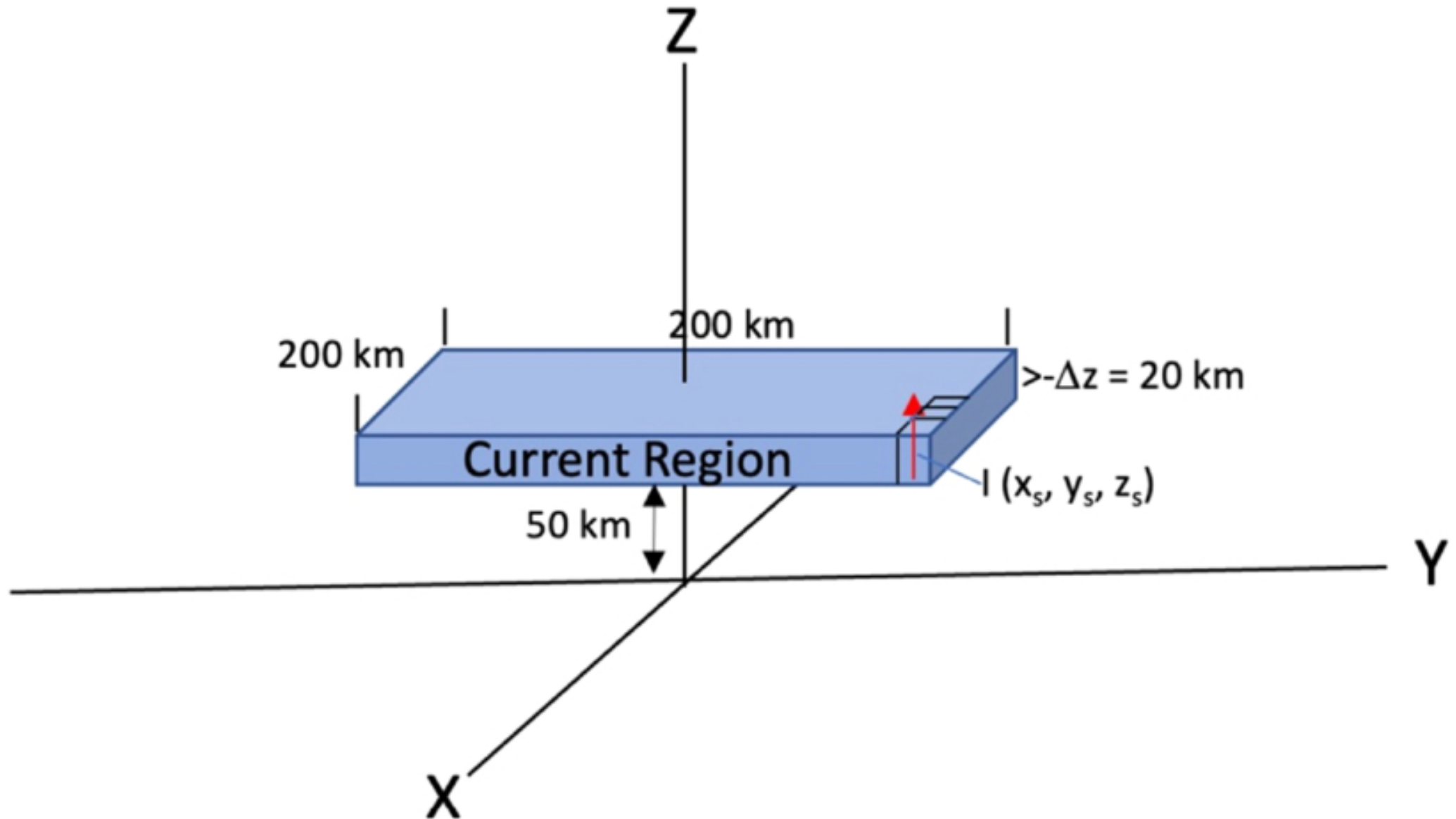
Figure 9. from William M. Farrell et al 2026 Planet. Sci. J. 7 doi:10.3847/PSJ/ae8c39 https://dx.doi.org/10.3847/PSJ/ae8c39 © 2026. The Author(s). Published by the American Astronomical Society.
