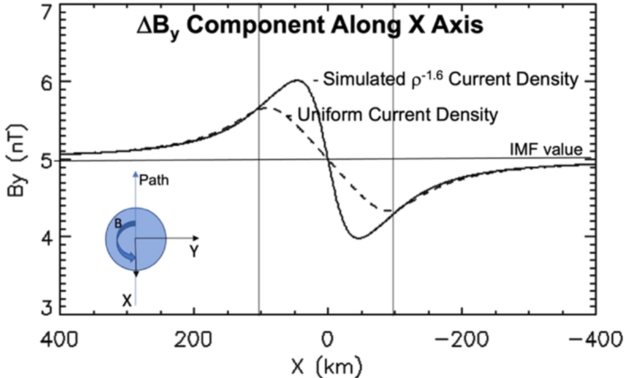
Figure 8. from William M. Farrell et al 2026 Planet. Sci. J. 7 doi:10.3847/PSJ/ae8c39 https://dx.doi.org/10.3847/PSJ/ae8c39 © 2026. The Author(s). Published by the American Astronomical Society.
