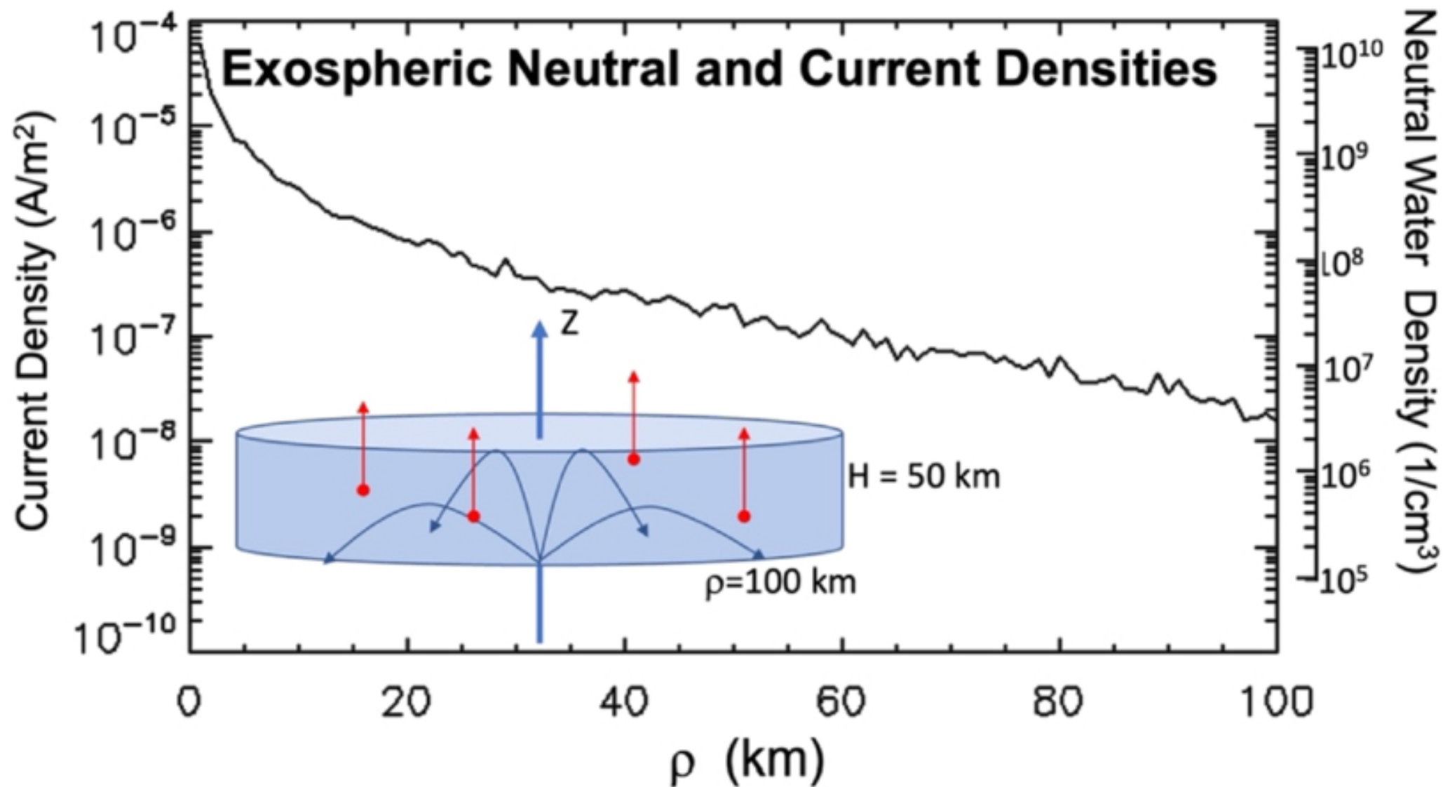
Figure 7. from William M. Farrell et al 2026 Planet. Sci. J. 7 doi:10.3847/PSJ/ae8c39 https://dx.doi.org/10.3847/PSJ/ae8c39 © 2026. The Author(s). Published by the American Astronomical Society.
