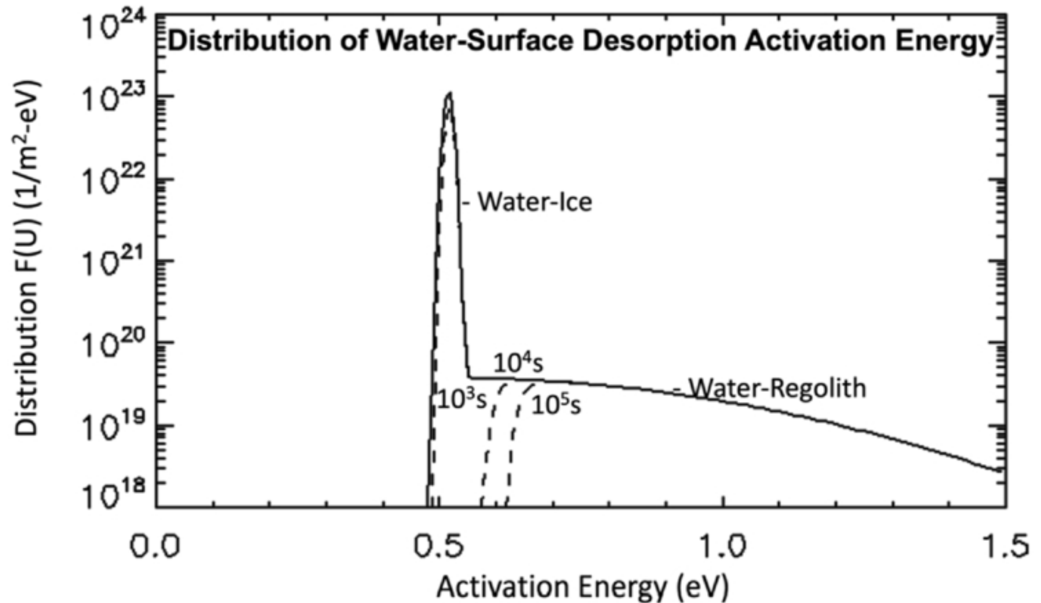
Figure 3. from William M. Farrell et al 2026 Planet. Sci. J. 7 doi:10.3847/PSJ/ae8c39 https://dx.doi.org/10.3847/PSJ/ae8c39 © 2026. The Author(s). Published by the American Astronomical Society.
