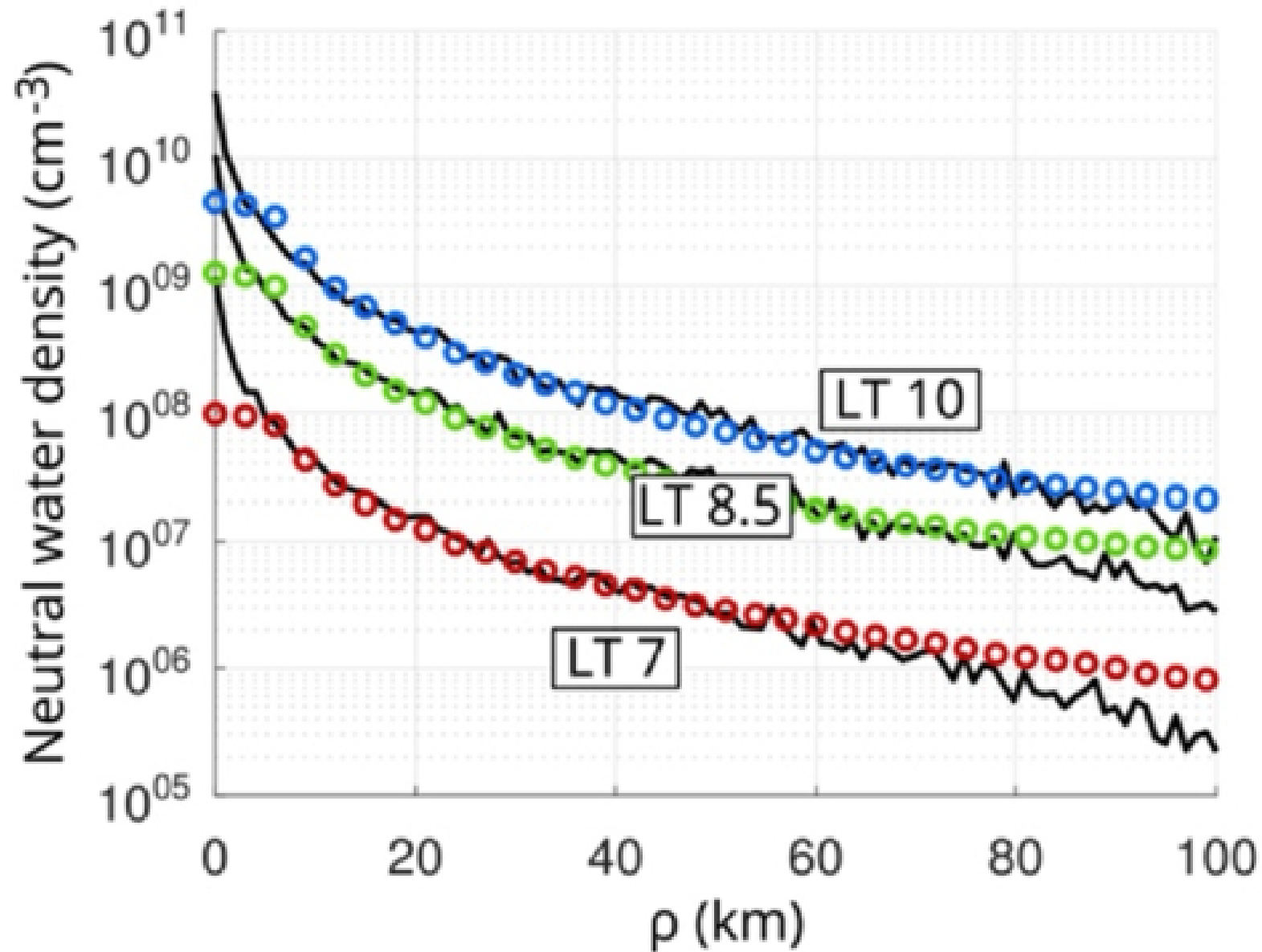
Figure A2. from William M. Farrell et al 2026 Planet. Sci. J. 7 doi:10.3847/PSJ/ae8c39 https://dx.doi.org/10.3847/PSJ/ae8c39 © 2026. The Author(s). Published by the American Astronomical Society.
