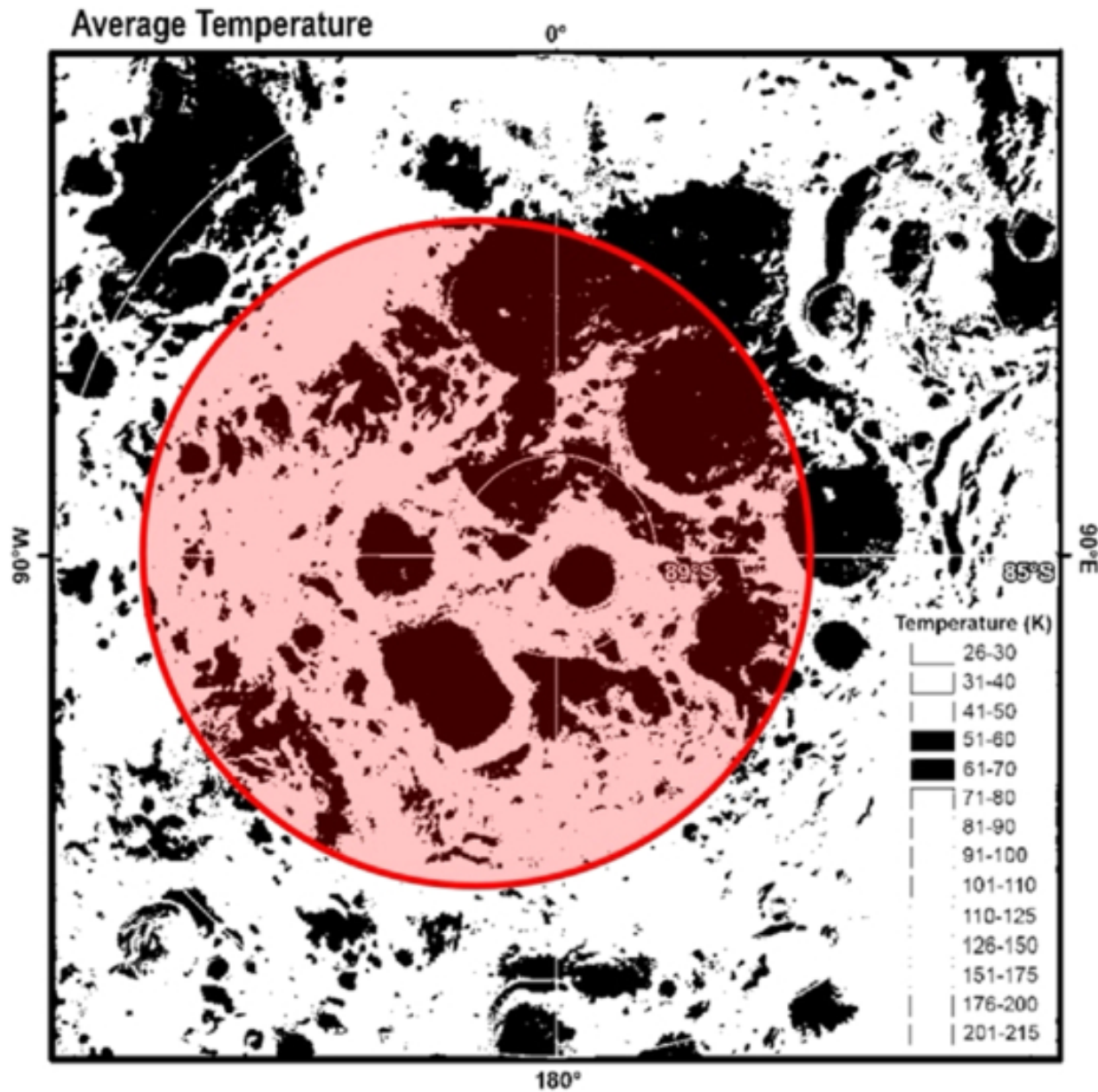
Figure 10. from William M. Farrell et al 2026 Planet. Sci. J. 7 doi:10.3847/PSJ/ae8c39 https://dx.doi.org/10.3847/PSJ/ae8c39 © 2026. The Author(s). Published by the American Astronomical Society.
