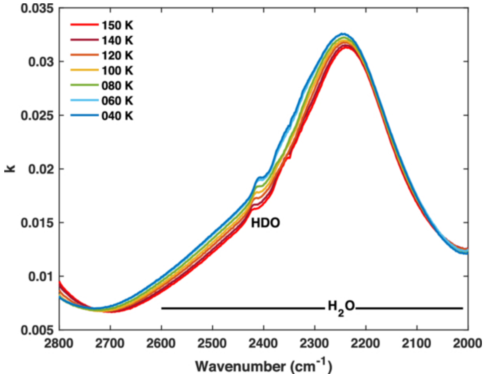
Figure 9. from Stephen C. Tegler et al 2026 Planet. Sci. J. 7 doi:10.3847/PSJ/ae8c34 https://dx.doi.org/10.3847/PSJ/ae8c34 © 2026. The Author(s). Published by the American Astronomical Society.
