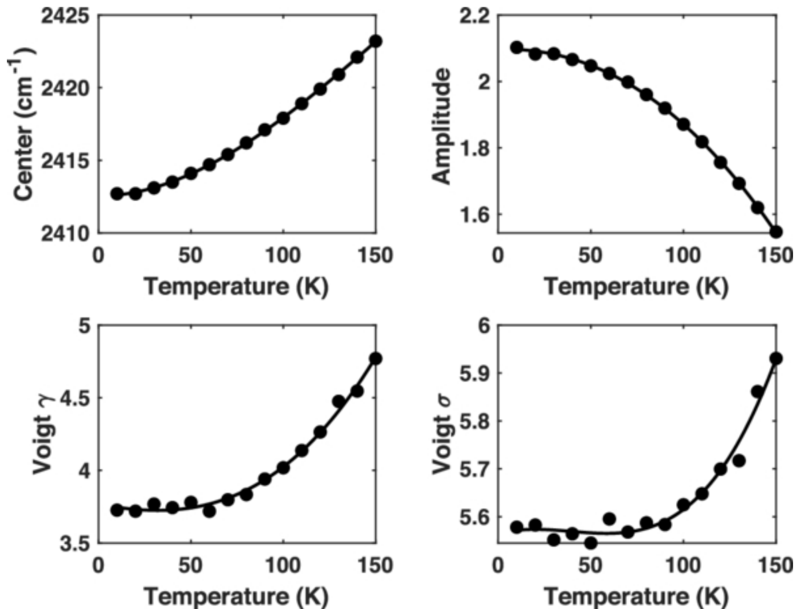
Figure 8. from Stephen C. Tegler et al 2026 Planet. Sci. J. 7 doi:10.3847/PSJ/ae8c34 https://dx.doi.org/10.3847/PSJ/ae8c34 © 2026. The Author(s). Published by the American Astronomical Society.
