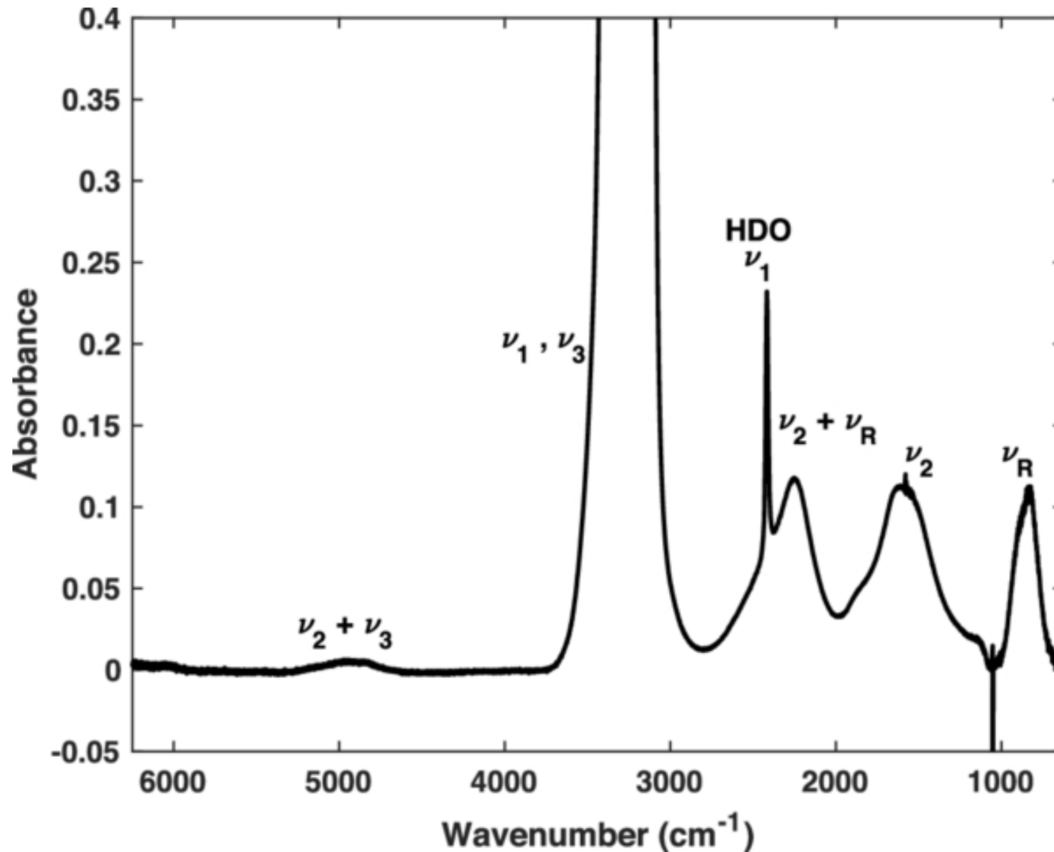
Figure 4. from Stephen C. Tegler et al 2026 Planet. Sci. J. 7 doi:10.3847/PSJ/ae8c34 https://dx.doi.org/10.3847/PSJ/ae8c34 © 2026. The Author(s). Published by the American Astronomical Society.
