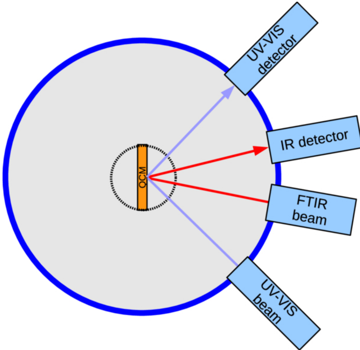
Figure 2. from Stephen C. Tegler et al 2026 Planet. Sci. J. 7 doi:10.3847/PSJ/ae8c34 https://dx.doi.org/10.3847/PSJ/ae8c34 © 2026. The Author(s). Published by the American Astronomical Society.
