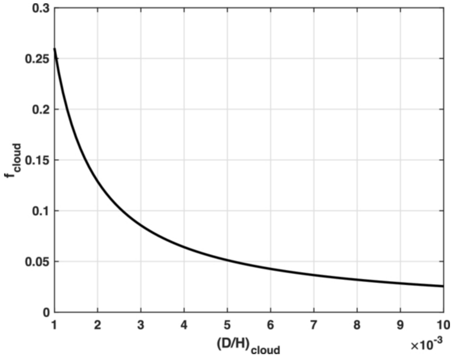
Figure 14. from Stephen C. Tegler et al 2026 Planet. Sci. J. 7 doi:10.3847/PSJ/ae8c34 https://dx.doi.org/10.3847/PSJ/ae8c34 © 2026. The Author(s). Published by the American Astronomical Society.
