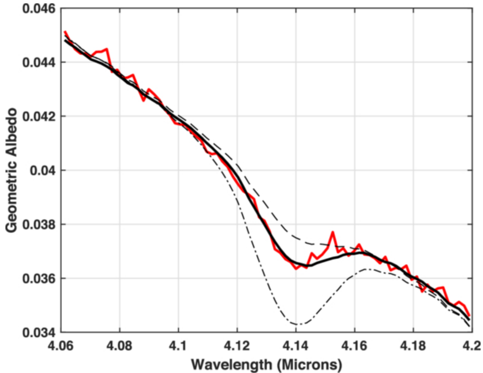
Figure 12. from Stephen C. Tegler et al 2026 Planet. Sci. J. 7 doi:10.3847/PSJ/ae8c34 https://dx.doi.org/10.3847/PSJ/ae8c34 © 2026. The Author(s). Published by the American Astronomical Society.
