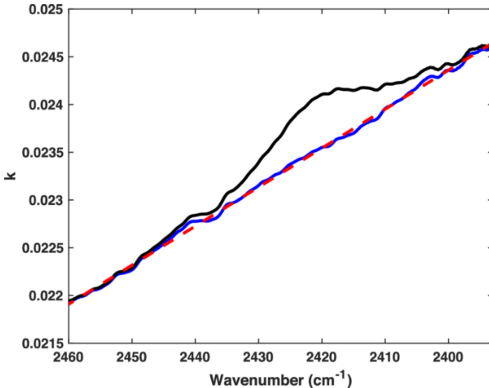
Figure 11. from Stephen C. Tegler et al 2026 Planet. Sci. J. 7 doi:10.3847/PSJ/ae8c34 https://dx.doi.org/10.3847/PSJ/ae8c34 © 2026. The Author(s). Published by the American Astronomical Society.
