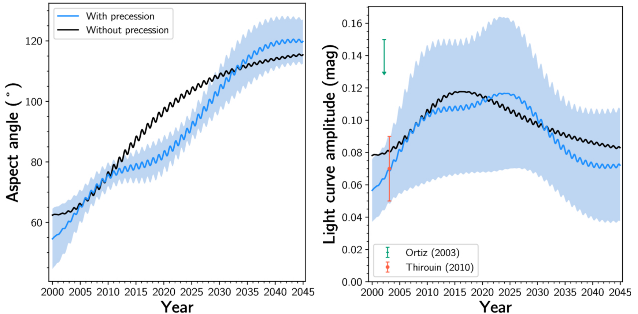
Figure 4. from Benjamin Proudfoot et al 2026 Planet. Sci. J. 7 doi:10.3847/PSJ/ae8ba5 https://dx.doi.org/10.3847/PSJ/ae8ba5 © 2026. The Author(s). Published by the American Astronomical Society.
