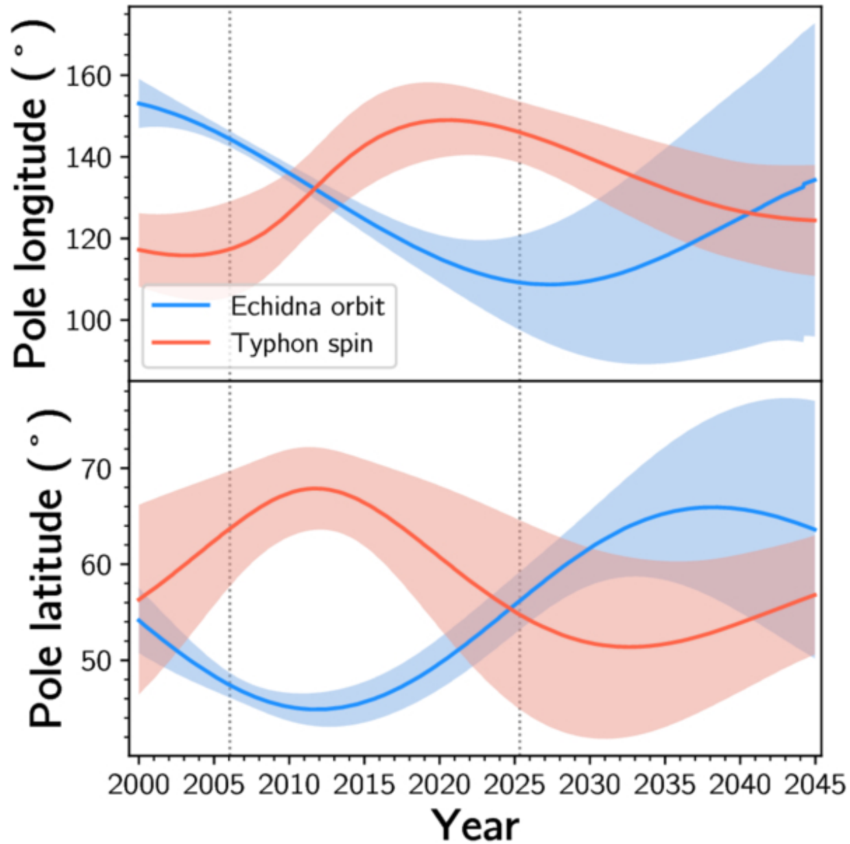
Figure 3. from Benjamin Proudfoot et al 2026 Planet. Sci. J. 7 doi:10.3847/PSJ/ae8ba5 https://dx.doi.org/10.3847/PSJ/ae8ba5 © 2026. The Author(s). Published by the American Astronomical Society.
