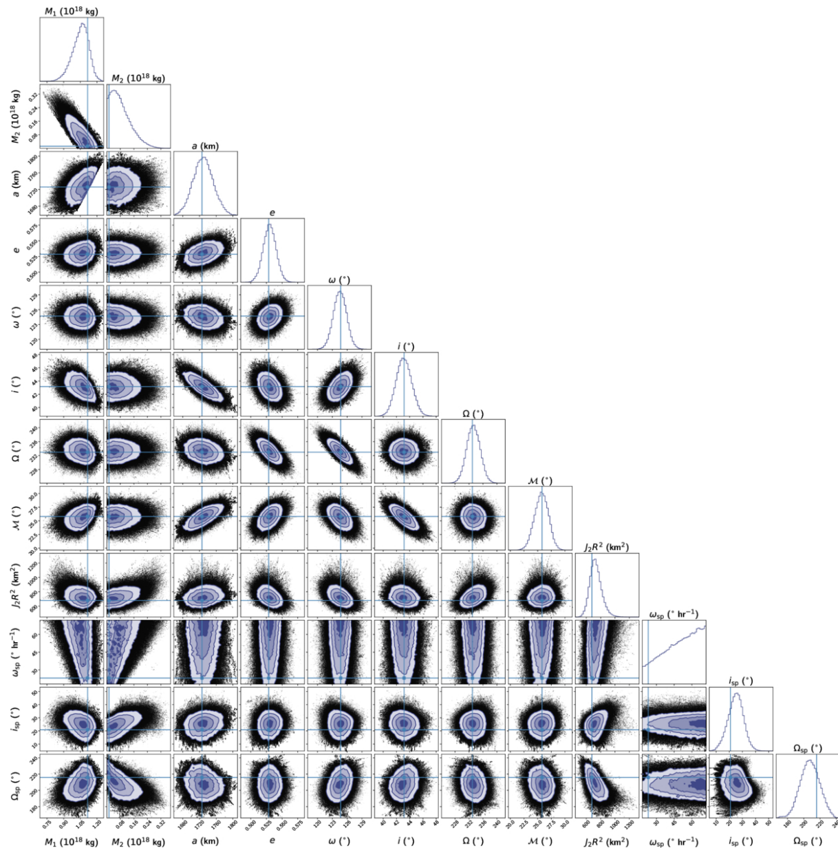
Figure 1. from Benjamin Proudfoot et al 2026 Planet. Sci. J. 7 doi:10.3847/PSJ/ae8ba5 https://dx.doi.org/10.3847/PSJ/ae8ba5 © 2026. The Author(s). Published by the American Astronomical Society.
