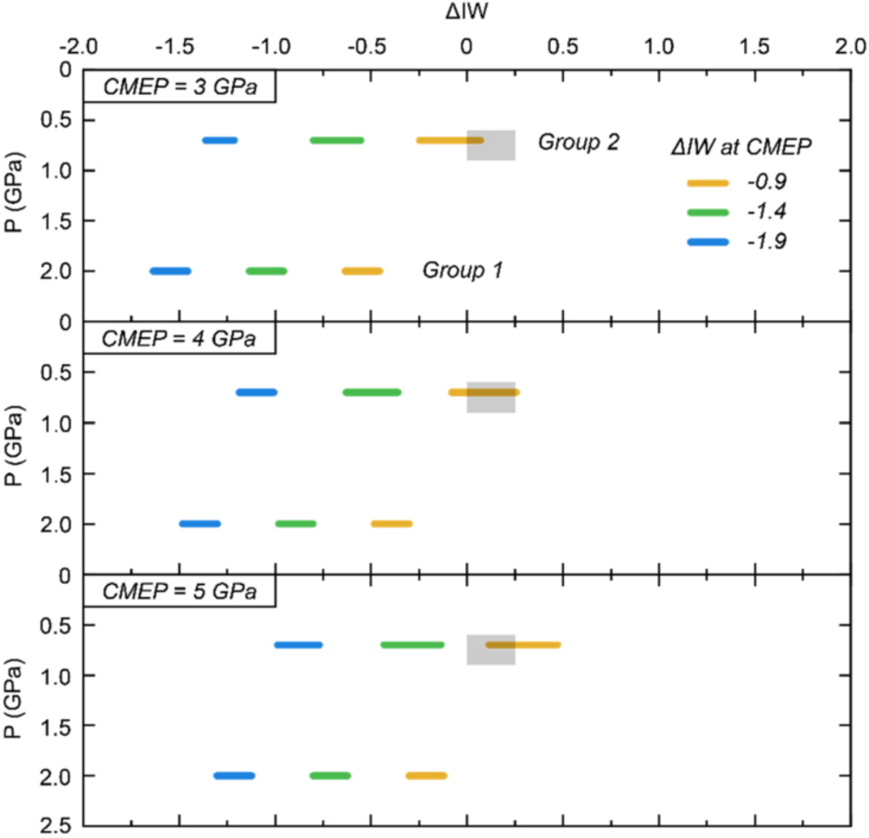
Figure A3. from Hideharu Kuwahara et al 2026 Planet. Sci. J. 7 doi:10.3847/PSJ/ae8ba4 https://dx.doi.org/10.3847/PSJ/ae8ba4 © 2026. The Author(s). Published by the American Astronomical Society.
