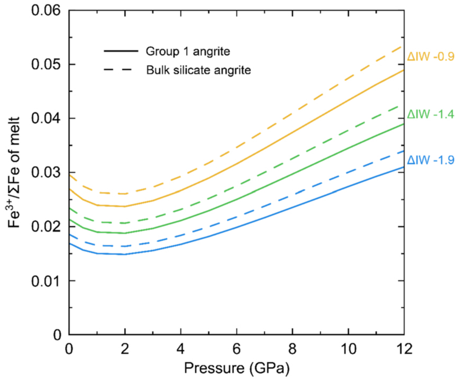
Figure A2. from Hideharu Kuwahara et al 2026 Planet. Sci. J. 7 doi:10.3847/PSJ/ae8ba4 https://dx.doi.org/10.3847/PSJ/ae8ba4 © 2026. The Author(s). Published by the American Astronomical Society.
