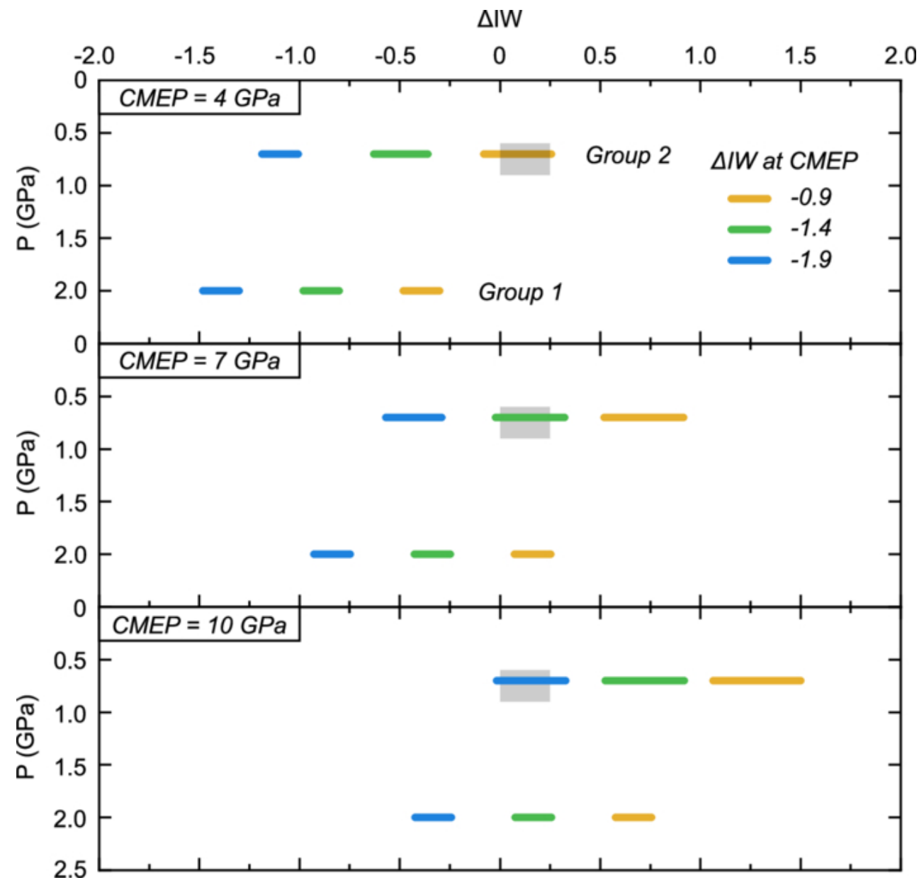
Figure 4. from Hideharu Kuwahara et al 2026 Planet. Sci. J. 7 doi:10.3847/PSJ/ae8ba4 https://dx.doi.org/10.3847/PSJ/ae8ba4 © 2026. The Author(s). Published by the American Astronomical Society.
