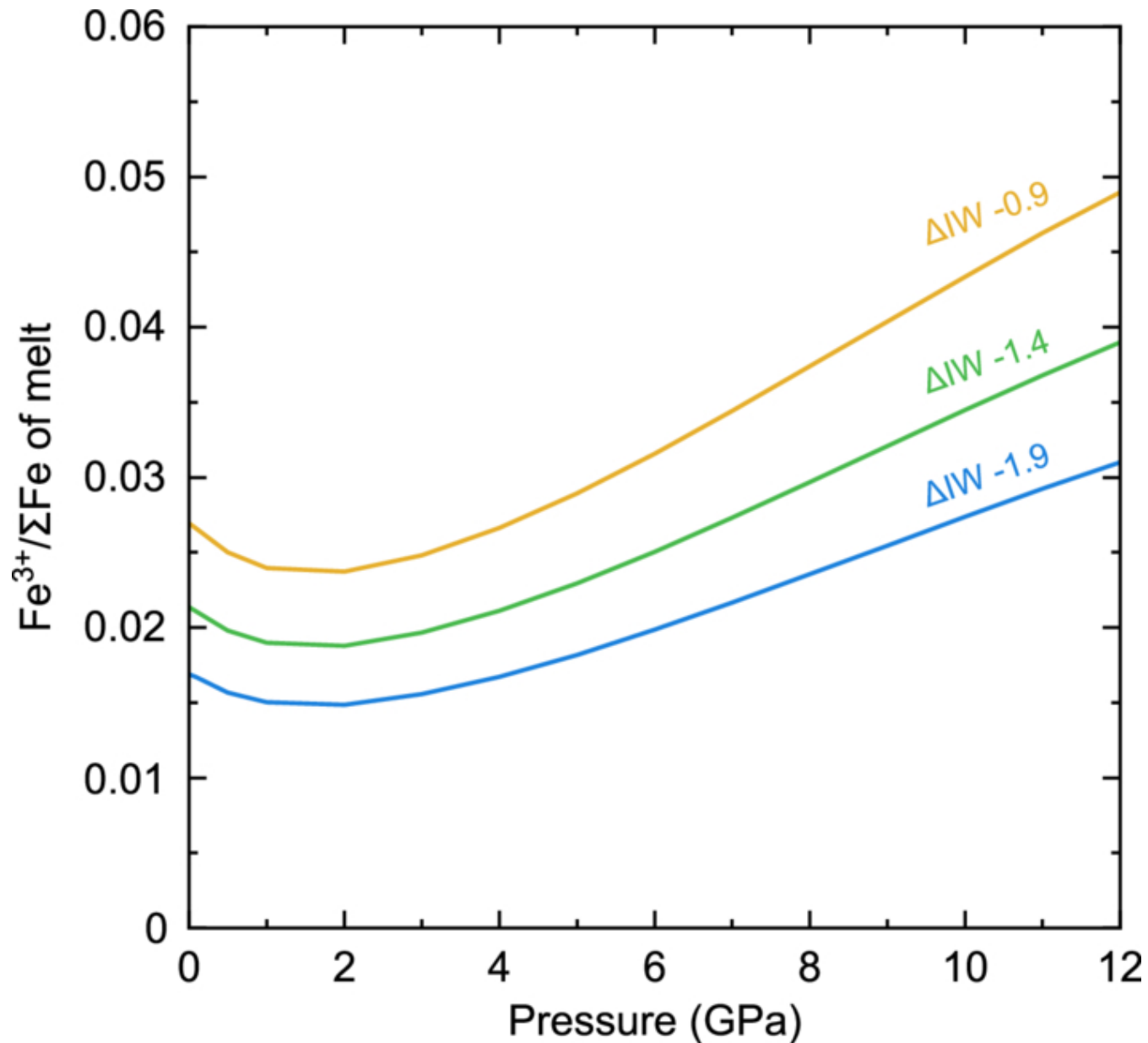
Figure 2. from Hideharu Kuwahara et al 2026 Planet. Sci. J. 7 doi:10.3847/PSJ/ae8ba4 https://dx.doi.org/10.3847/PSJ/ae8ba4 © 2026. The Author(s). Published by the American Astronomical Society.
