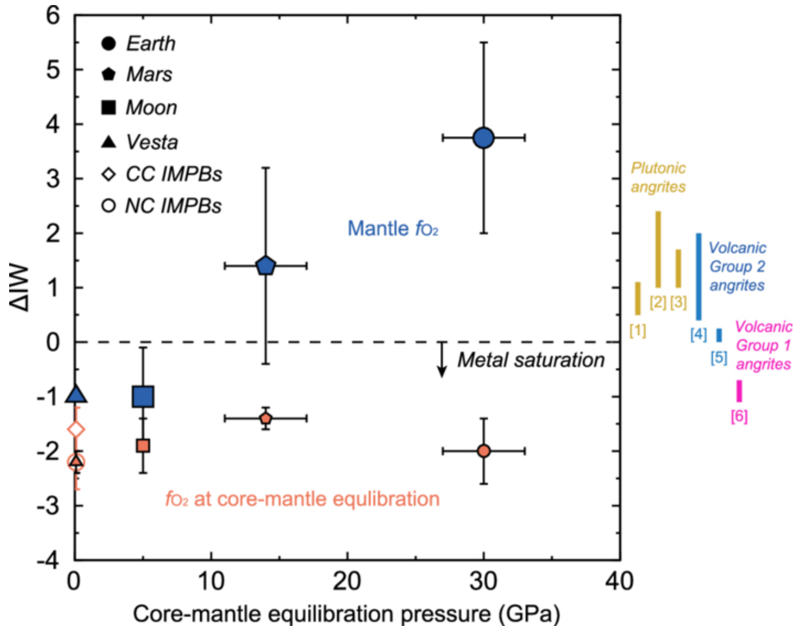
Figure 1. from Hideharu Kuwahara et al 2026 Planet. Sci. J. 7 doi:10.3847/PSJ/ae8ba4 https://dx.doi.org/10.3847/PSJ/ae8ba4 © 2026. The Author(s). Published by the American Astronomical Society.
