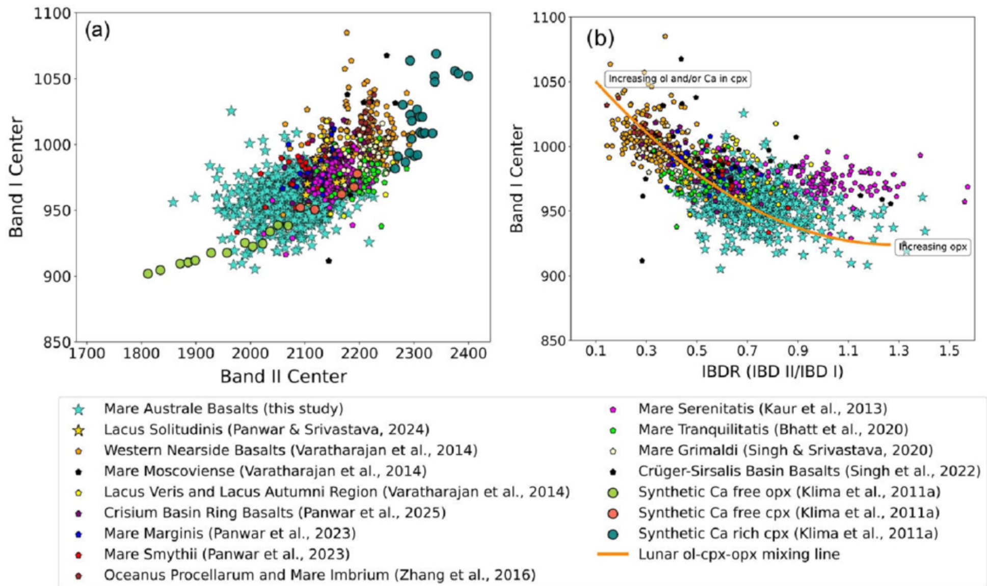
Figure 4. from Neha Panwar et al 2026 Planet. Sci. J. 7 doi:10.3847/PSJ/ae8ba3 https://dx.doi.org/10.3847/PSJ/ae8ba3 © 2026. The Author(s). Published by the American Astronomical Society.
