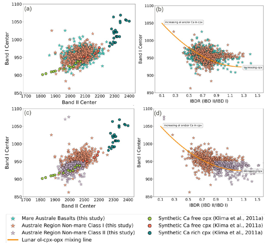
Figure 3. from Neha Panwar et al 2026 Planet. Sci. J. 7 doi:10.3847/PSJ/ae8ba3 https://dx.doi.org/10.3847/PSJ/ae8ba3 © 2026. The Author(s). Published by the American Astronomical Society.
