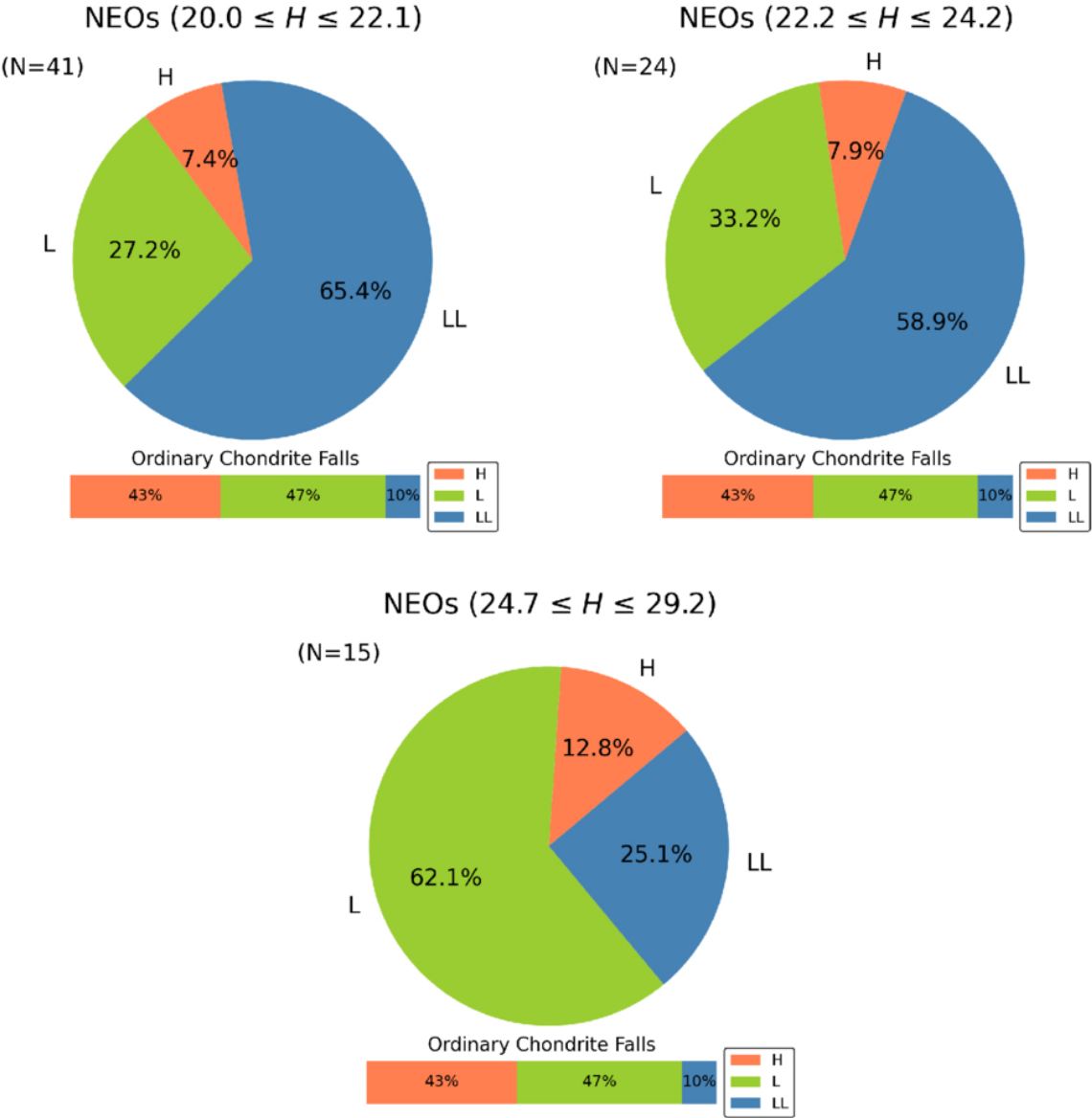
Figure 8. from Juan A. Sanchez et al 2026 Planet. Sci. J. 7 doi:10.3847/PSJ/ae8af0 https://dx.doi.org/10.3847/PSJ/ae8af0 © 2026. The Author(s). Published by the American Astronomical Society.
