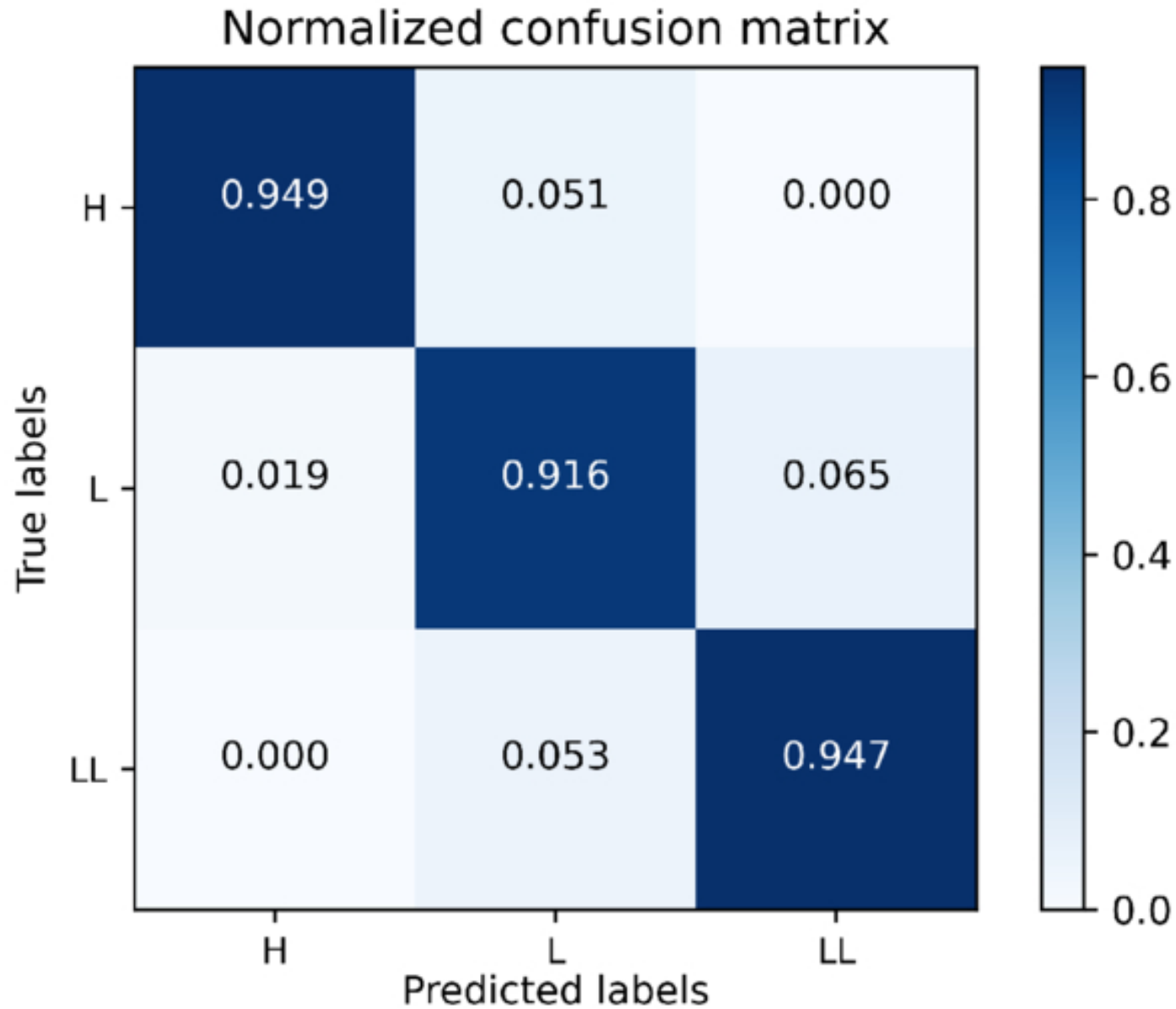
Figure 6. from Juan A. Sanchez et al 2026 Planet. Sci. J. 7 doi:10.3847/PSJ/ae8af0 https://dx.doi.org/10.3847/PSJ/ae8af0 © 2026. The Author(s). Published by the American Astronomical Society.
