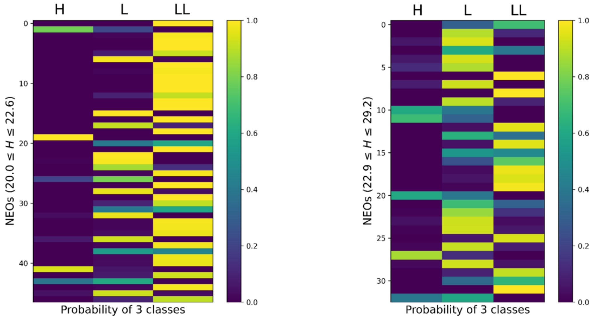
Figure 5. from Juan A. Sanchez et al 2026 Planet. Sci. J. 7 doi:10.3847/PSJ/ae8af0 https://dx.doi.org/10.3847/PSJ/ae8af0 © 2026. The Author(s). Published by the American Astronomical Society.
