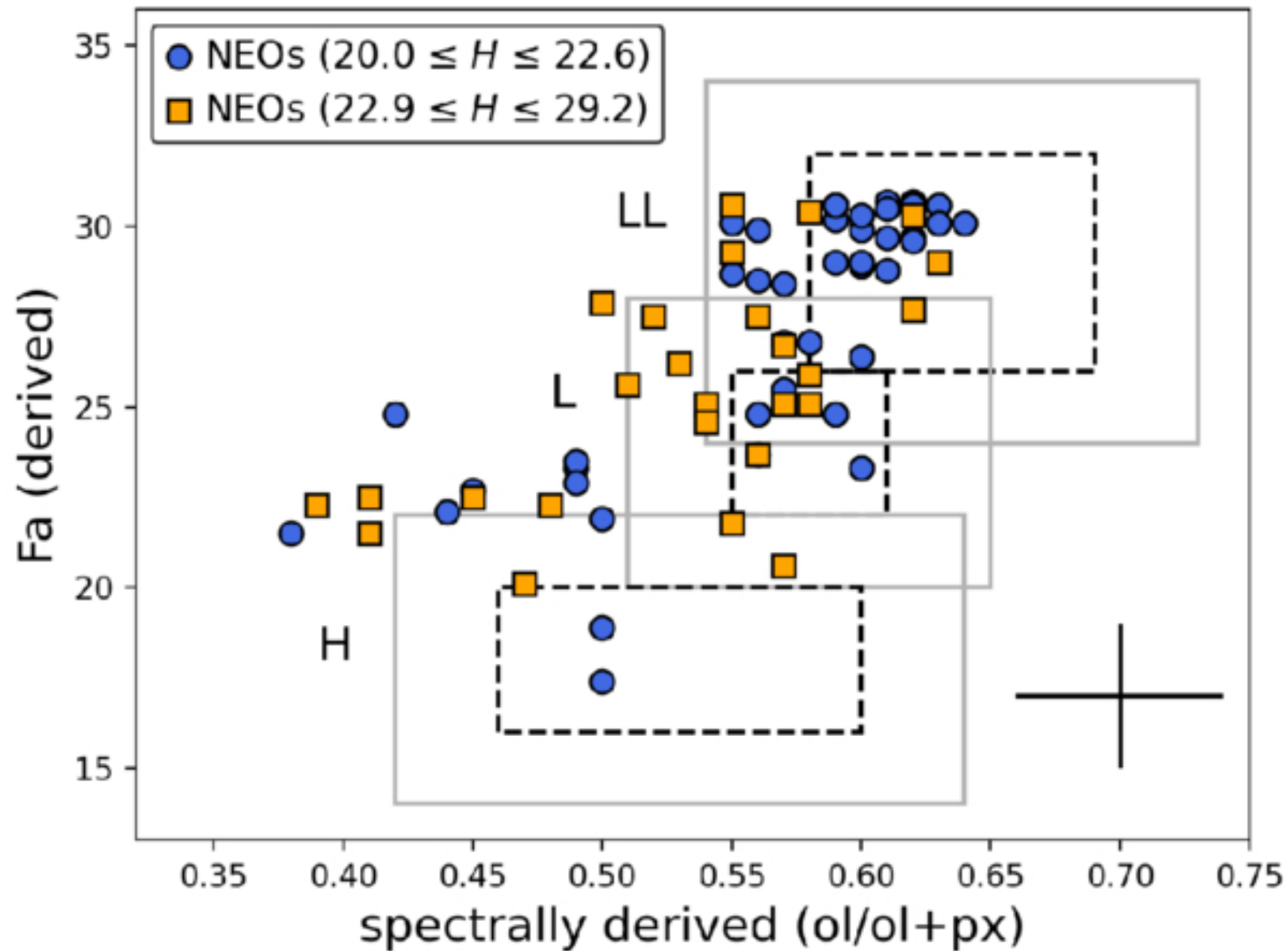
Figure 4. from Juan A. Sanchez et al 2026 Planet. Sci. J. 7 doi:10.3847/PSJ/ae8af0 https://dx.doi.org/10.3847/PSJ/ae8af0 © 2026. The Author(s). Published by the American Astronomical Society.
