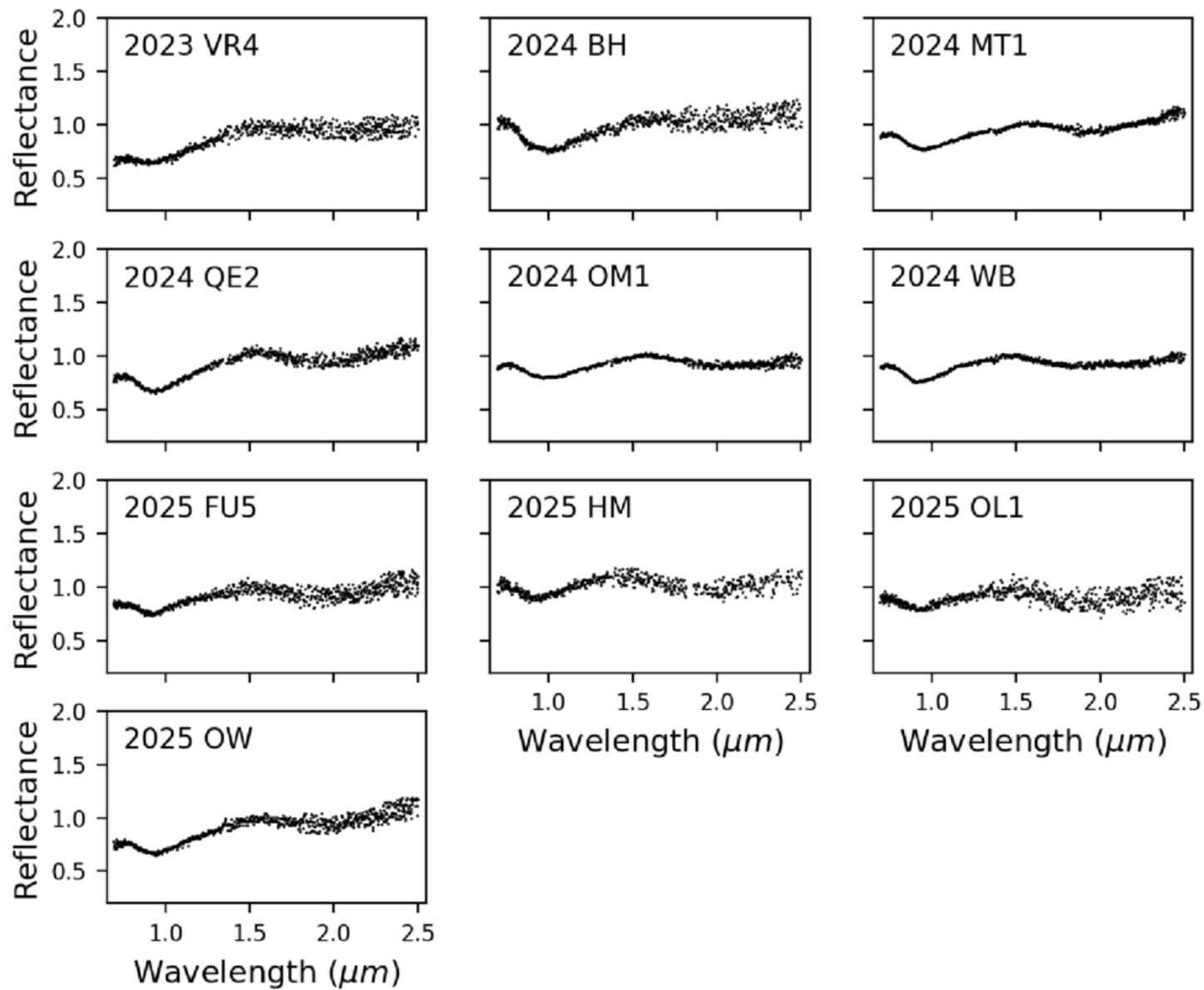
Figure 15. from Juan A. Sanchez et al 2026 Planet. Sci. J. 7 doi:10.3847/PSJ/ae8af0 https://dx.doi.org/10.3847/PSJ/ae8af0 © 2026. The Author(s). Published by the American Astronomical Society.
