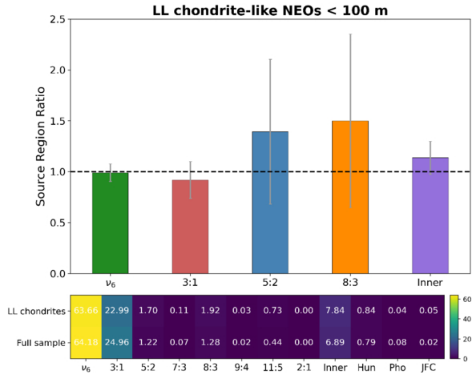
Figure 13. from Juan A. Sanchez et al 2026 Planet. Sci. J. 7 doi:10.3847/PSJ/ae8af0 https://dx.doi.org/10.3847/PSJ/ae8af0 © 2026. The Author(s). Published by the American Astronomical Society.
