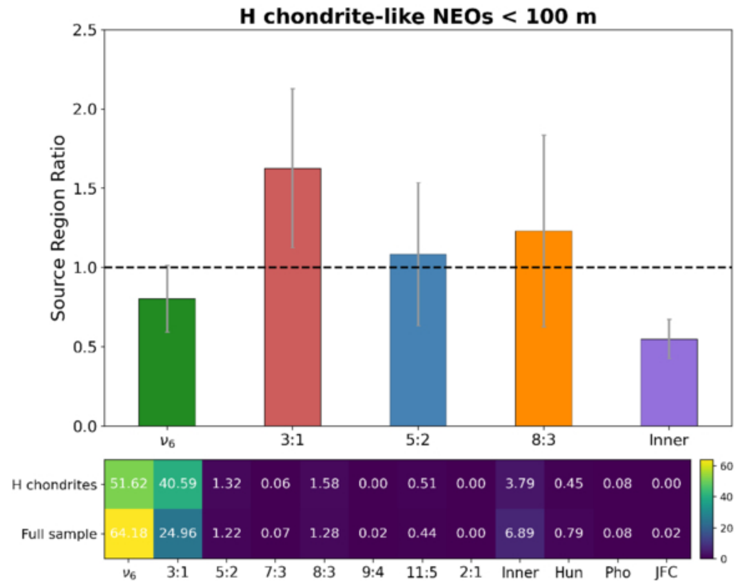
Figure 11. from Juan A. Sanchez et al 2026 Planet. Sci. J. 7 doi:10.3847/PSJ/ae8af0 https://dx.doi.org/10.3847/PSJ/ae8af0 © 2026. The Author(s). Published by the American Astronomical Society.
