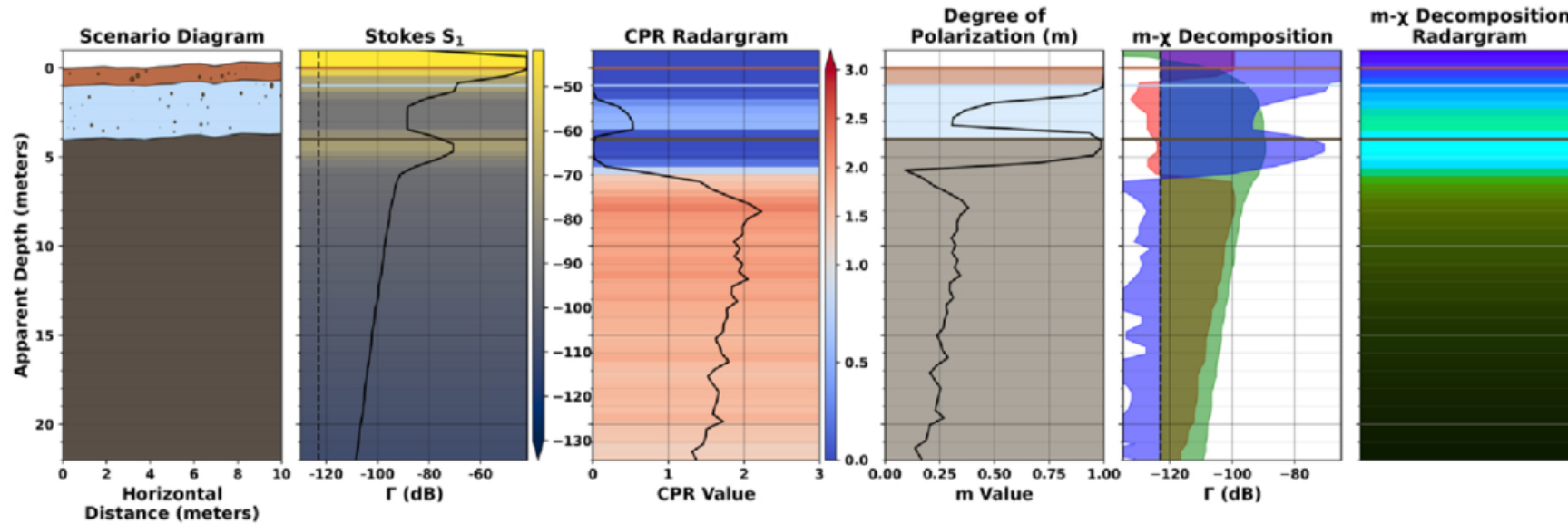
Figure 9. from Ivan Mishev et al 2026 Planet. Sci. J. 7 doi:10.3847/PSJ/ae8ae5 https://dx.doi.org/10.3847/PSJ/ae8ae5 © 2026. The Author(s). Published by the American Astronomical Society.
