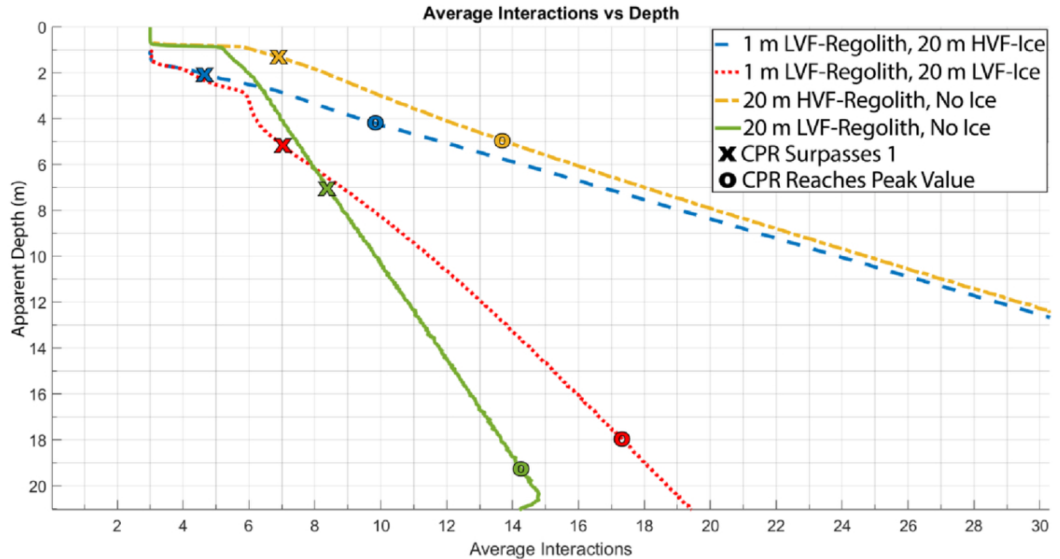
Figure 7. from Ivan Mishev et al 2026 Planet. Sci. J. 7 doi:10.3847/PSJ/ae8ae5 https://dx.doi.org/10.3847/PSJ/ae8ae5 © 2026. The Author(s). Published by the American Astronomical Society.
