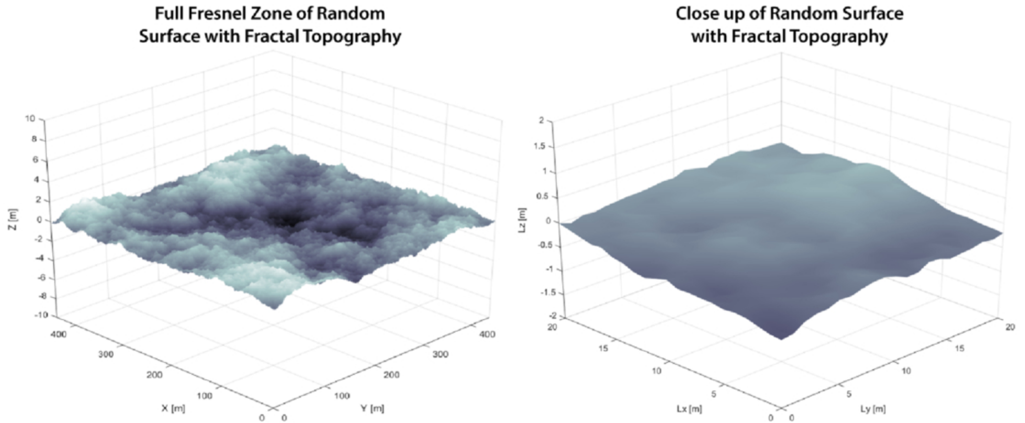
Figure 4. from Ivan Mishev et al 2026 Planet. Sci. J. 7 doi:10.3847/PSJ/ae8ae5 https://dx.doi.org/10.3847/PSJ/ae8ae5 © 2026. The Author(s). Published by the American Astronomical Society.
