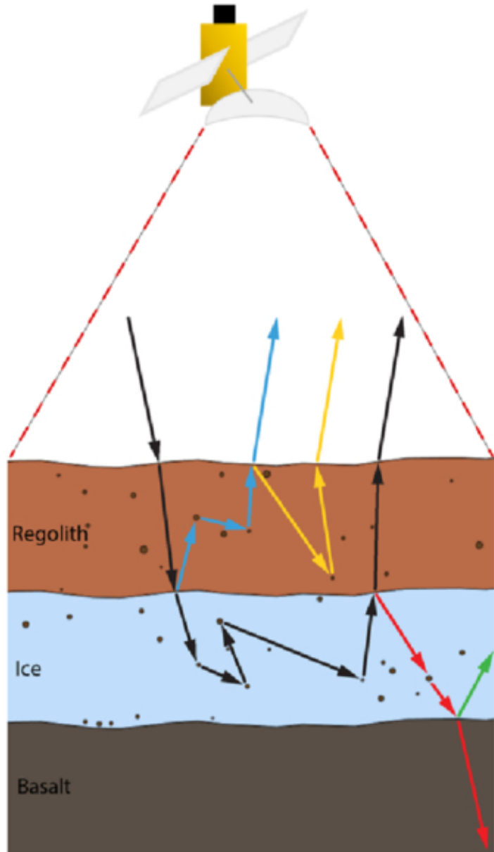
Figure 2. from Ivan Mishev et al 2026 Planet. Sci. J. 7 doi:10.3847/PSJ/ae8ae5 https://dx.doi.org/10.3847/PSJ/ae8ae5 © 2026. The Author(s). Published by the American Astronomical Society.
