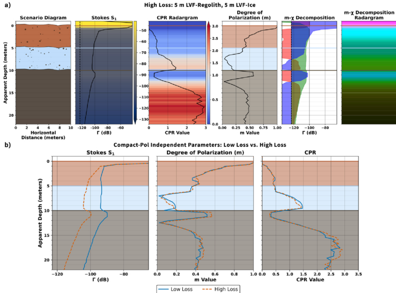
Figure 14. from Ivan Mishev et al 2026 Planet. Sci. J. 7 doi:10.3847/PSJ/ae8ae5 https://dx.doi.org/10.3847/PSJ/ae8ae5 © 2026. The Author(s). Published by the American Astronomical Society.
