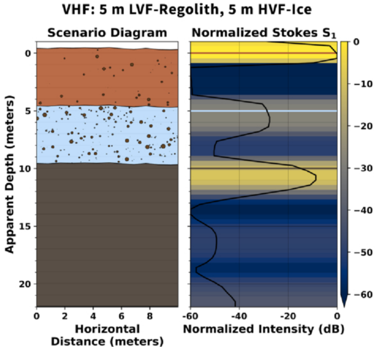
Figure 12. from Ivan Mishev et al 2026 Planet. Sci. J. 7 doi:10.3847/PSJ/ae8ae5 https://dx.doi.org/10.3847/PSJ/ae8ae5 © 2026. The Author(s). Published by the American Astronomical Society.
