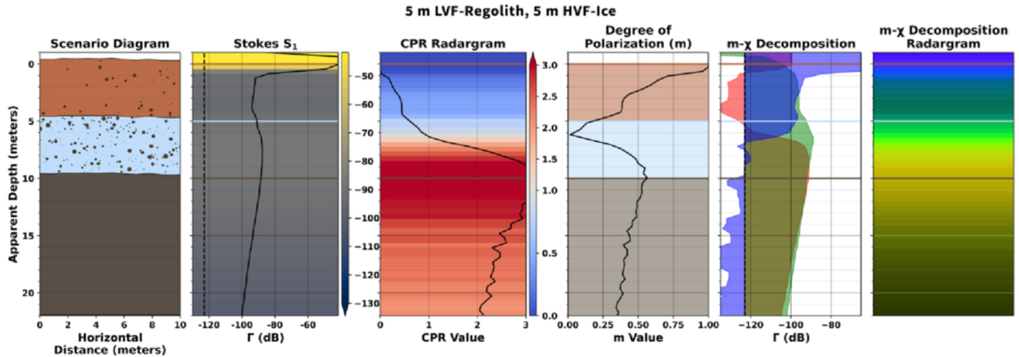
Figure 11. from Ivan Mishev et al 2026 Planet. Sci. J. 7 doi:10.3847/PSJ/ae8ae5 https://dx.doi.org/10.3847/PSJ/ae8ae5 © 2026. The Author(s). Published by the American Astronomical Society.
